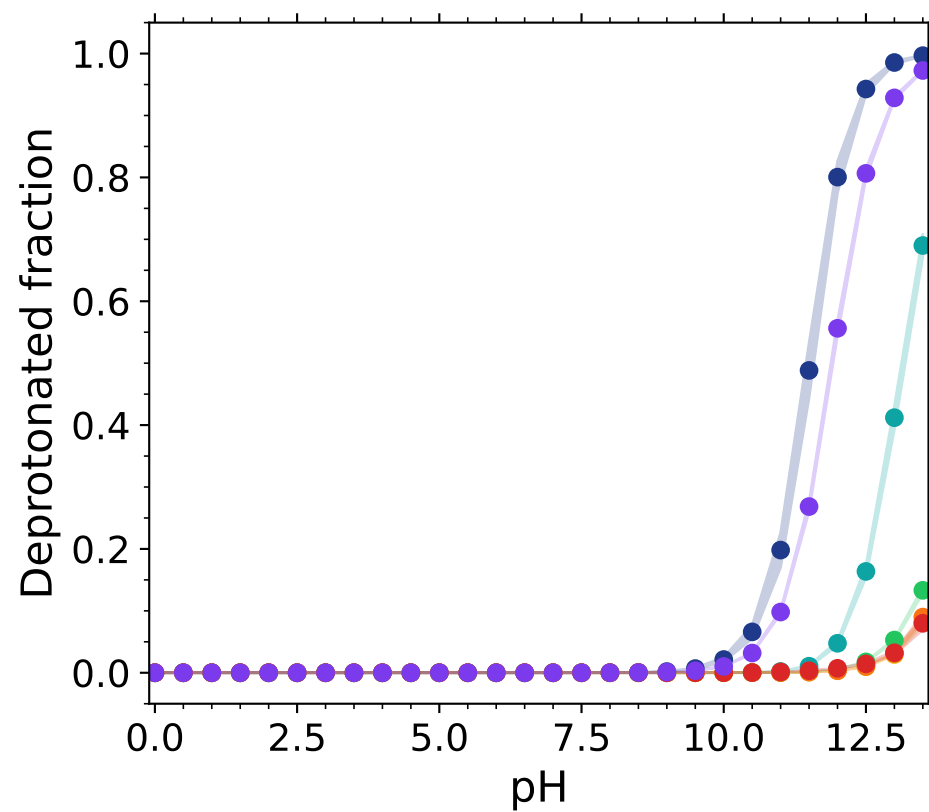
His B:5
