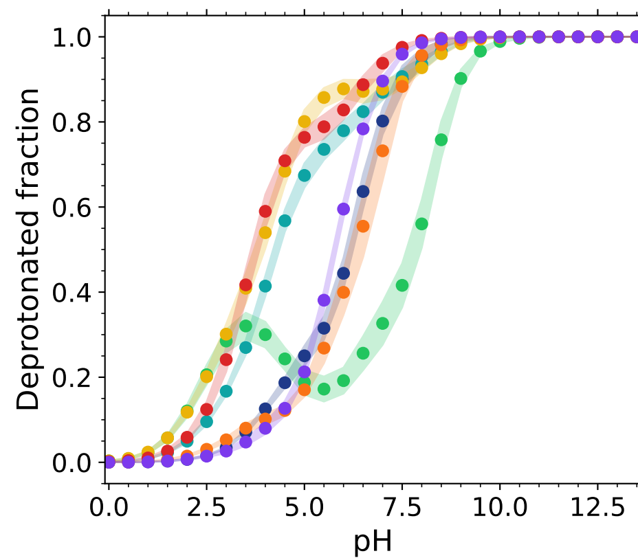
His B:10
