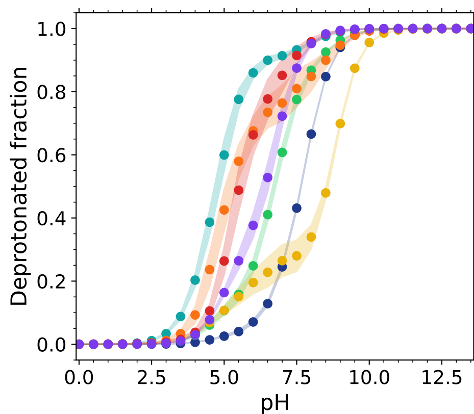
Tyr B:16
