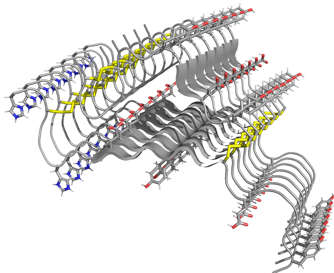
Heptameric insulin fibril
