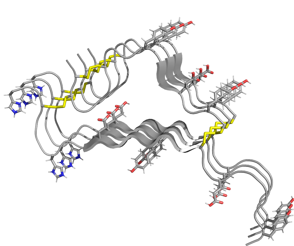
Trimeric insulin fibril
