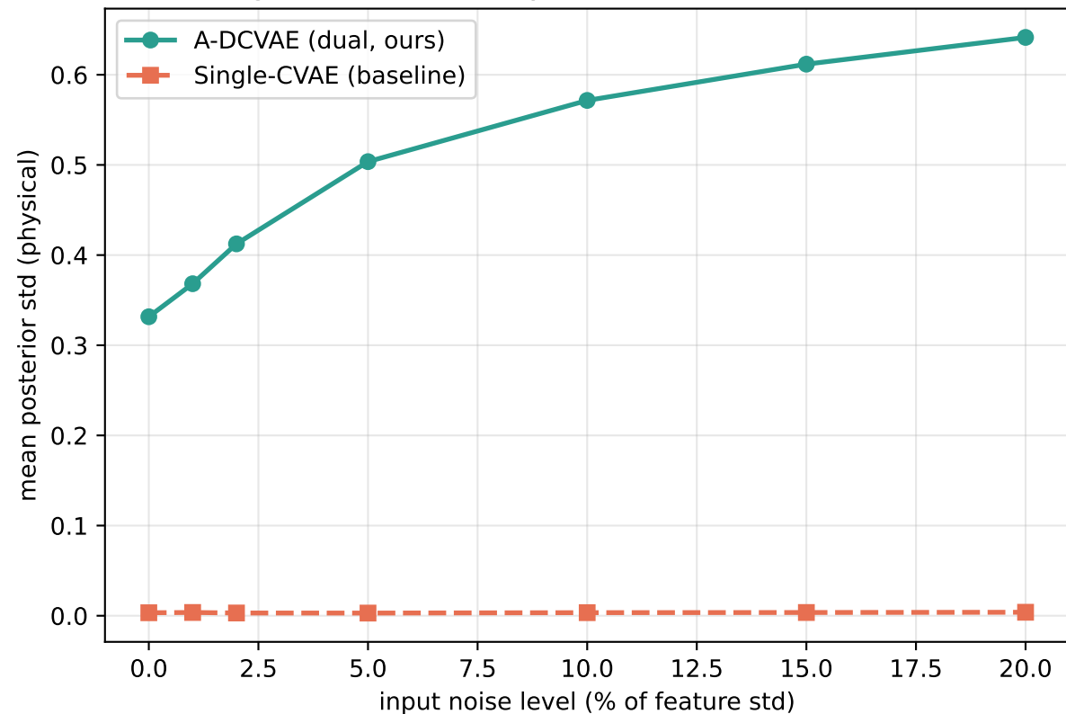
Fig 5: noise sensitivity — dual widens off-manifold
