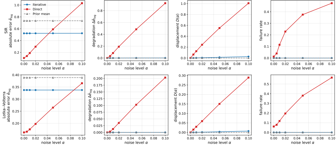
Figure 15: Test-time noise response for SIR (top) and Lotka–Volterra (bottom): absolute error, degradation, displacement, and failure rate versus \alpha . The same ordering as OGTT (Figure 13) holds: the direct regressor is most accurate when clean but degrades and violates support under noise, the iterative operator is flat at a higher floor, and the prior mean is flat and inaccurate. For LV the direct regressor already fails on 6% of clean test samples — a reflection of the exact prey-only ambiguity of Section 7.2, which places part of the fiber outside the training support even before noise.
