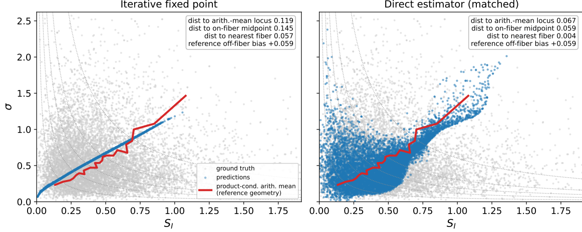
Figure 10: Predictions and the product-conditioned arithmetic-mean locus \tilde{m}(c) = \hat{\mathbb{E}}[(S_I, \sigma) \mid S_I\sigma = c] in the (S_I, \sigma) plane (shared test split; grey: ground-truth joint, dotted: constant- S_I\sigma fibers, red: \tilde{m}(c) ). The red curve is a reference geometry , not the estimators’ Bayes target: the network trains in log coordinates, whose on-fiber geometric mean — not this arithmetic locus — is its target (Remark 5.13), and \tilde{m}(c) conditions on the product rather than on \mathbf{x}_{\text{obs}} . Left : the iterative fixed point collapses onto a tight 1-D band, sitting off the fibers by an amount consistent with operator approximation. Right : the matched direct estimator recovers the product and fans along the fibers (near the on-fiber geometric mean). Annotations report per-bin distances and the off-fiber product bias \tilde{m}_1\tilde{m}_2 - c of the reference locus (positive, the Jensen property of Corollary 5.12 under physical-coordinate averaging).
