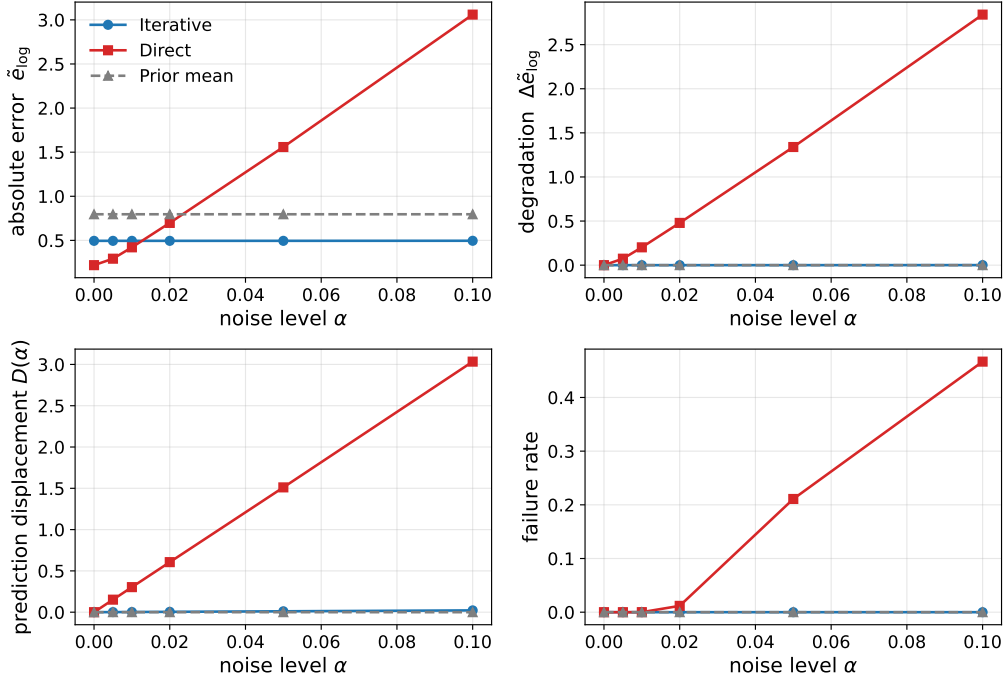
Figure 13: OGTT test-time noise response. ( Top left ) absolute error \tilde{e}_{\log} : the direct regressor is most accurate on clean data but crosses the flat prior-mean line near \alpha \approx 0.02 and keeps rising, while the iterative estimator stays flat at a higher floor. ( Top right ) clean-to-noisy degradation; ( bottom left ) prediction displacement; ( bottom right ) failure rate. Only the unbounded direct regressor degrades; the tanh-bounded iterative operator and the constant prior mean do not. Lower is better throughout.
