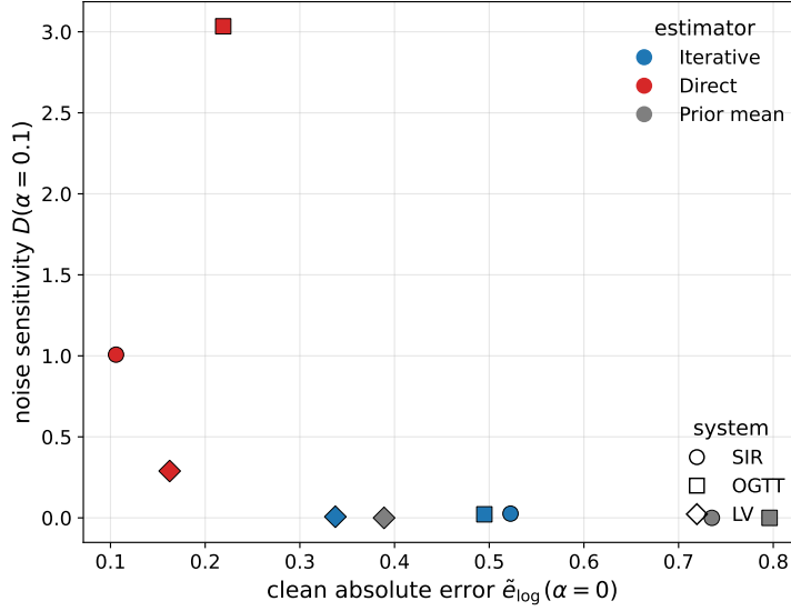
Figure 14: Stability–accuracy plane: clean absolute error (lower is more accurate) versus perturbation sensitivity D at \alpha = 0.10 (lower is more stable). The direct regressor occupies the accurate-but- sensitive corner, the prior mean the stable-but-inaccurate corner, and the iterative operator an intermediate, stable-but-biased position. No estimator reaches the ideal lower-left; the axes trade off.
