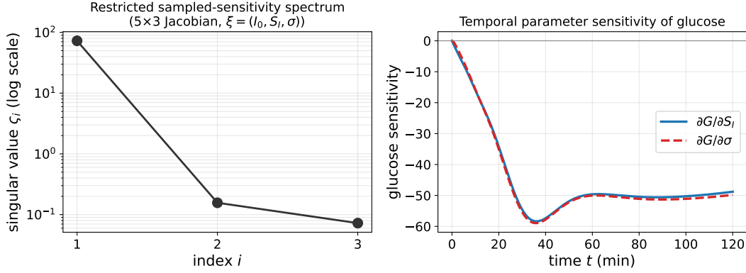
Figure 4: Restricted sampled sensitivity of the OGTT model. (Left) The three singular values of the 5 \times 3 Jacobian \nabla_{\xi} \mathcal{G} , \xi = (I_0, S_I, \sigma) , at the five-point grid: locally full rank 3 but spanning \sim 10^3 (ill-conditioned). (Right) The temporal sensitivity of glucose to S_I and \sigma is nearly identical throughout the window — the two parameters act on glucose almost interchangeably, so only their stiff combination is well determined.
