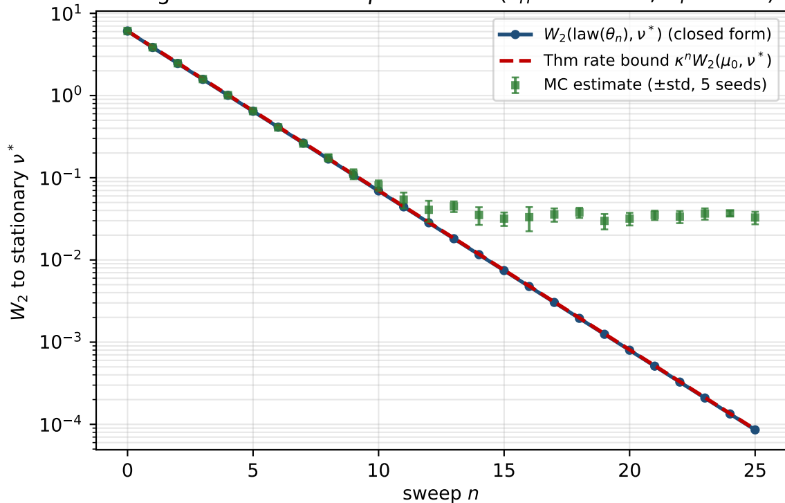
E-a: geometric rate \kappa = \rho^2 = 0.640 ( L_H = 1.60 > 1 , L_P = 0.40 )
