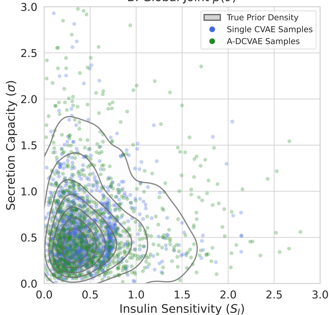
B. Global Joint p(\theta)
