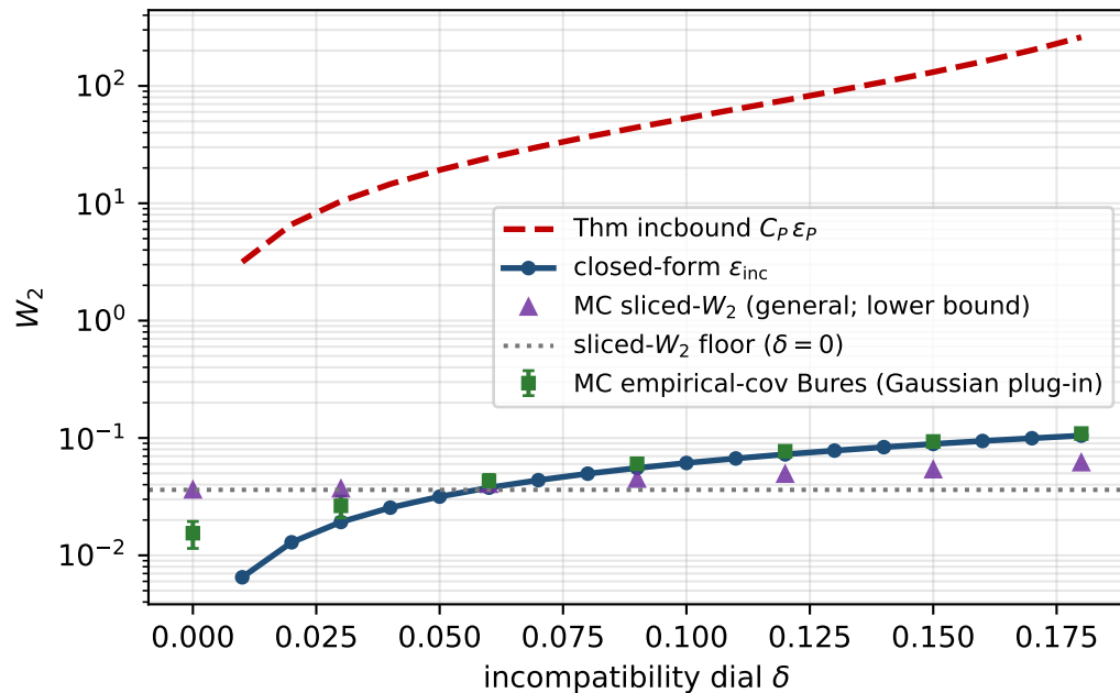
Panel B: self-consistency bound (Thm incbound)
