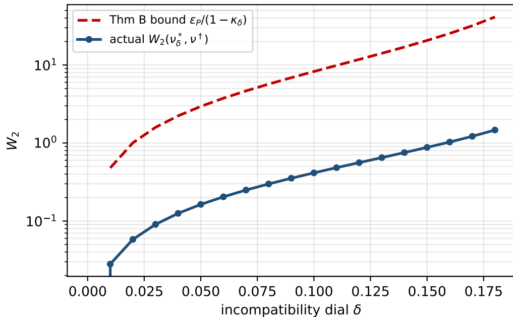
Panel A: steering bound (Thm B)
