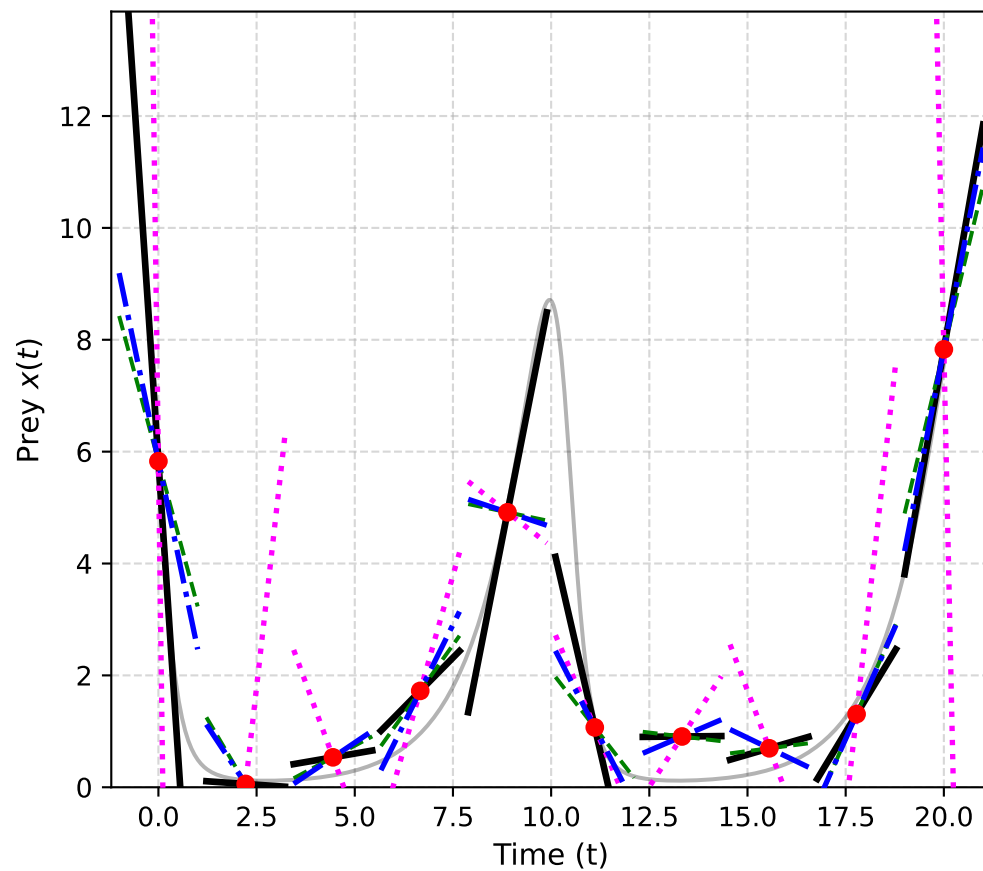
(b) Lotka-Volterra Model ( x )
