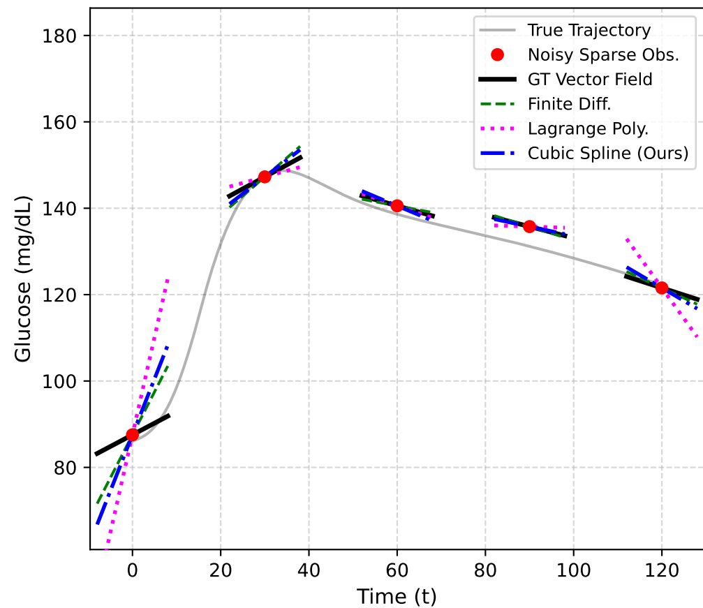
(c) OGTT Model ( G )
