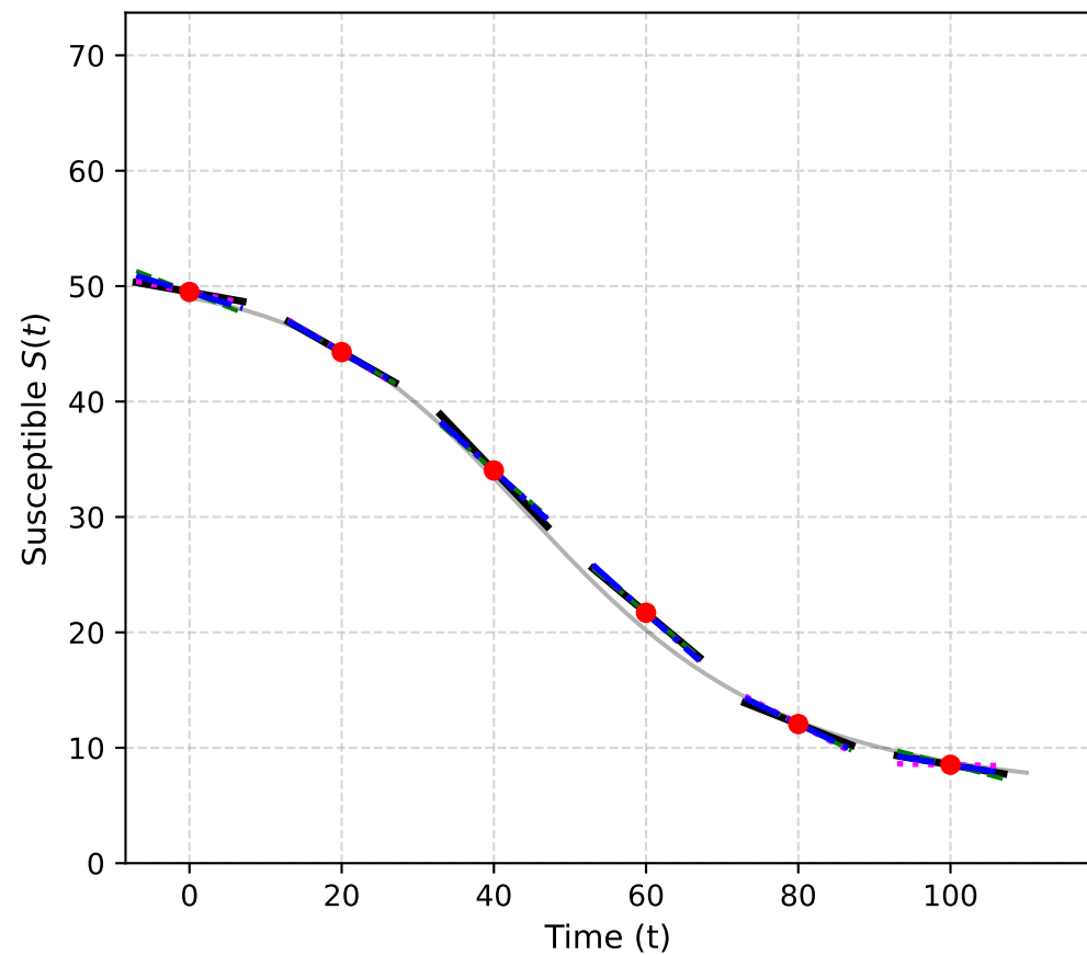
(a) SIR Model ( S )
