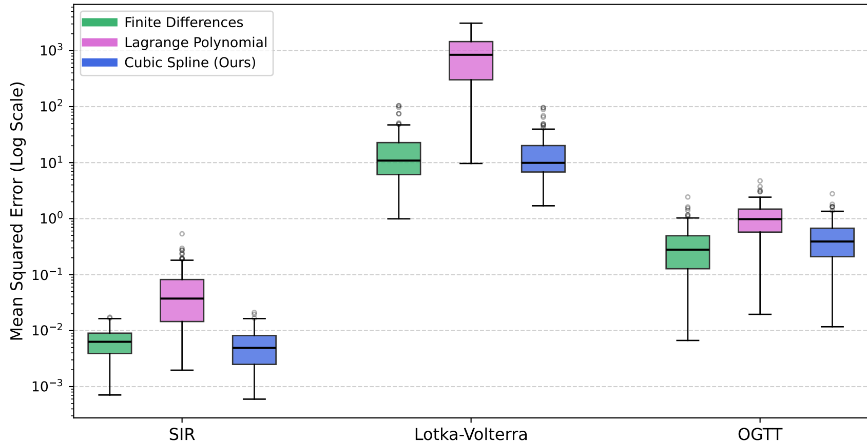
Robust Evaluation of Derivative Approximations ( N = 100 trajectories)
