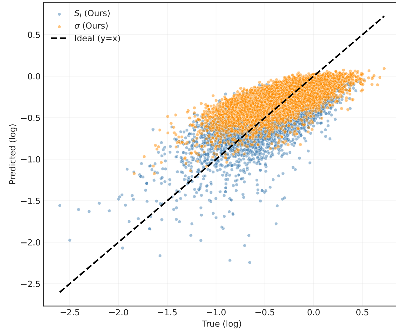
3. Individual coordinates S_l, \sigma (both sloppy)
