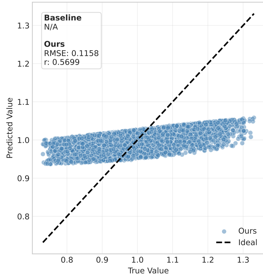
Basic Reproduction ( \mathcal{R}_0 )
