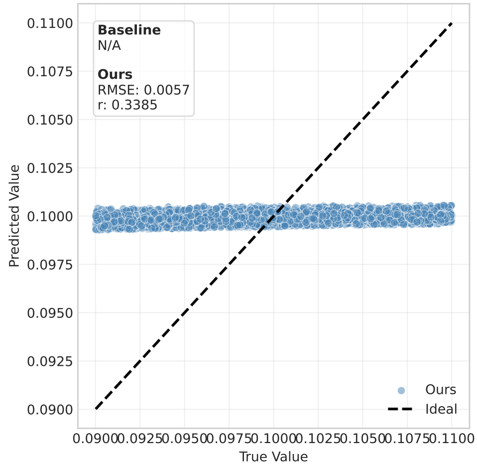
Recovery Rate ( \gamma )
