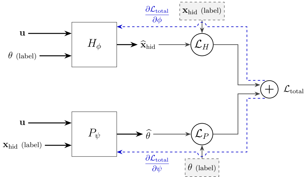
(a) Supervised training via teacher forcing
