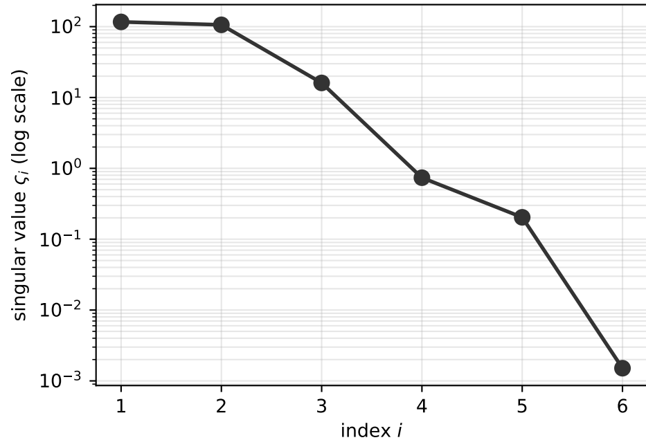
Observability Jacobian spectrum (decay \Rightarrow practical ill-conditioning)
