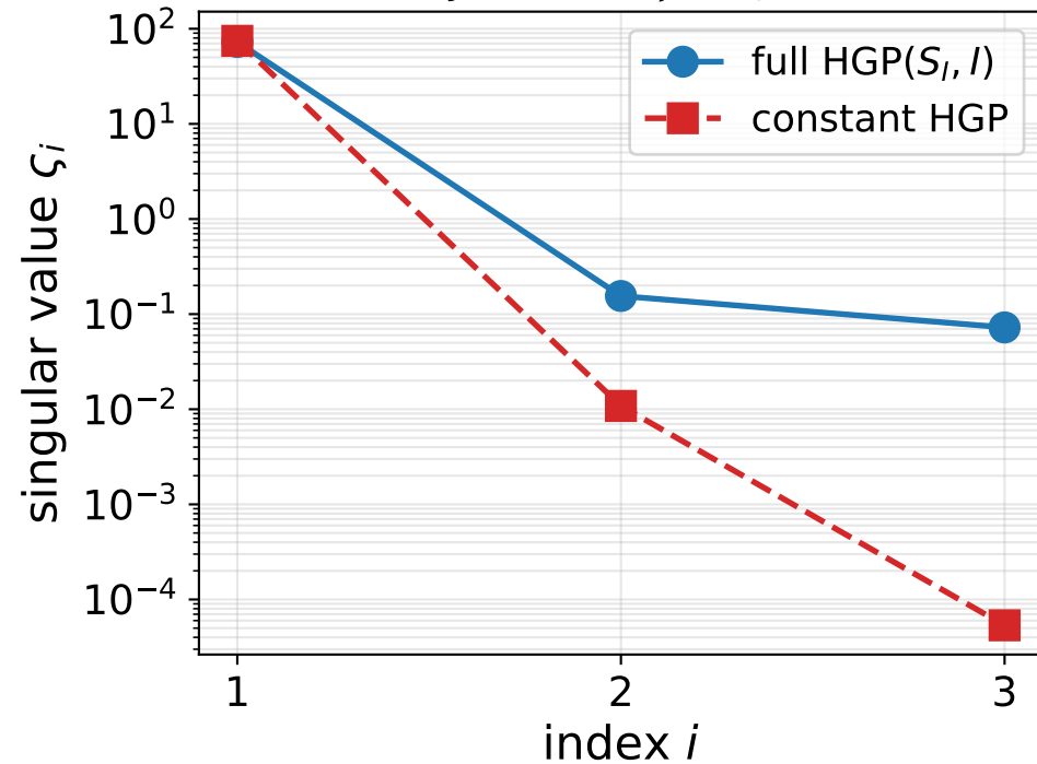
(a) Restricted spectrum 5×3 Jacobian, \xi = (I_0, S_I, \sigma)
