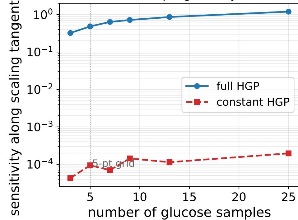
(b) Symmetry-breaking signal vs sampling density
