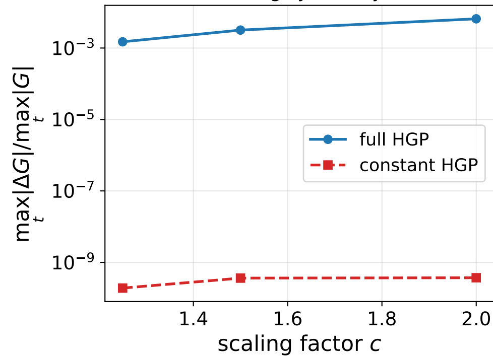
(c) Glucose invariance under the scaling symmetry
