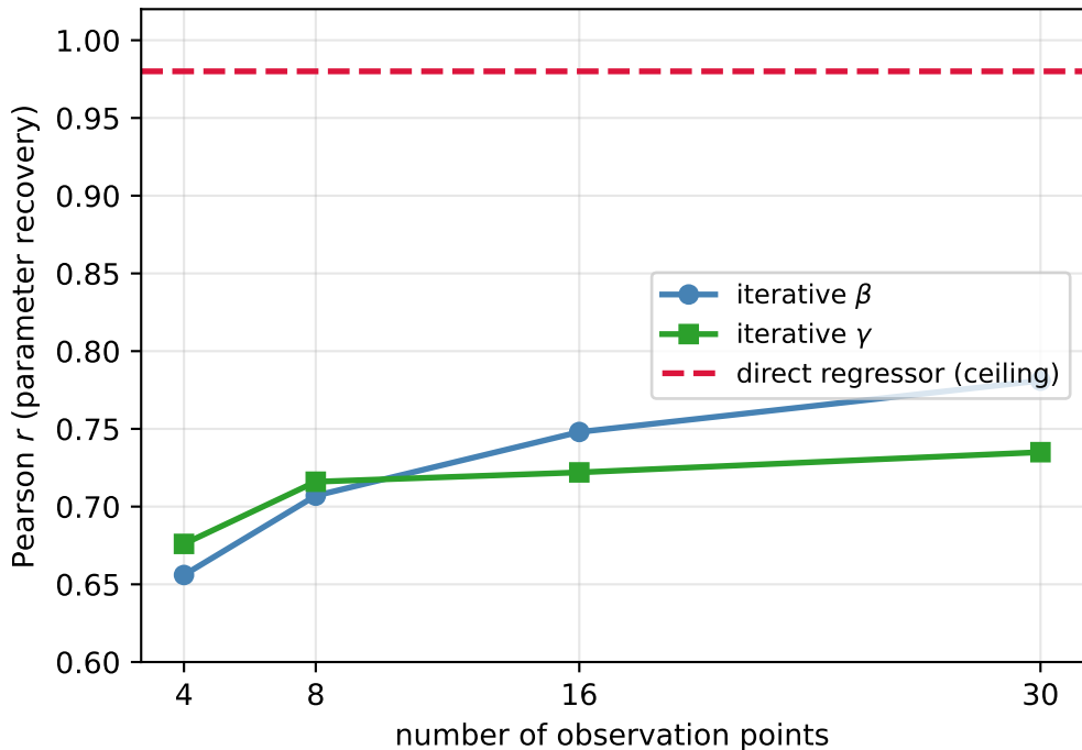
SIR: correctness improves with observation density but the reconstruction gap persists
