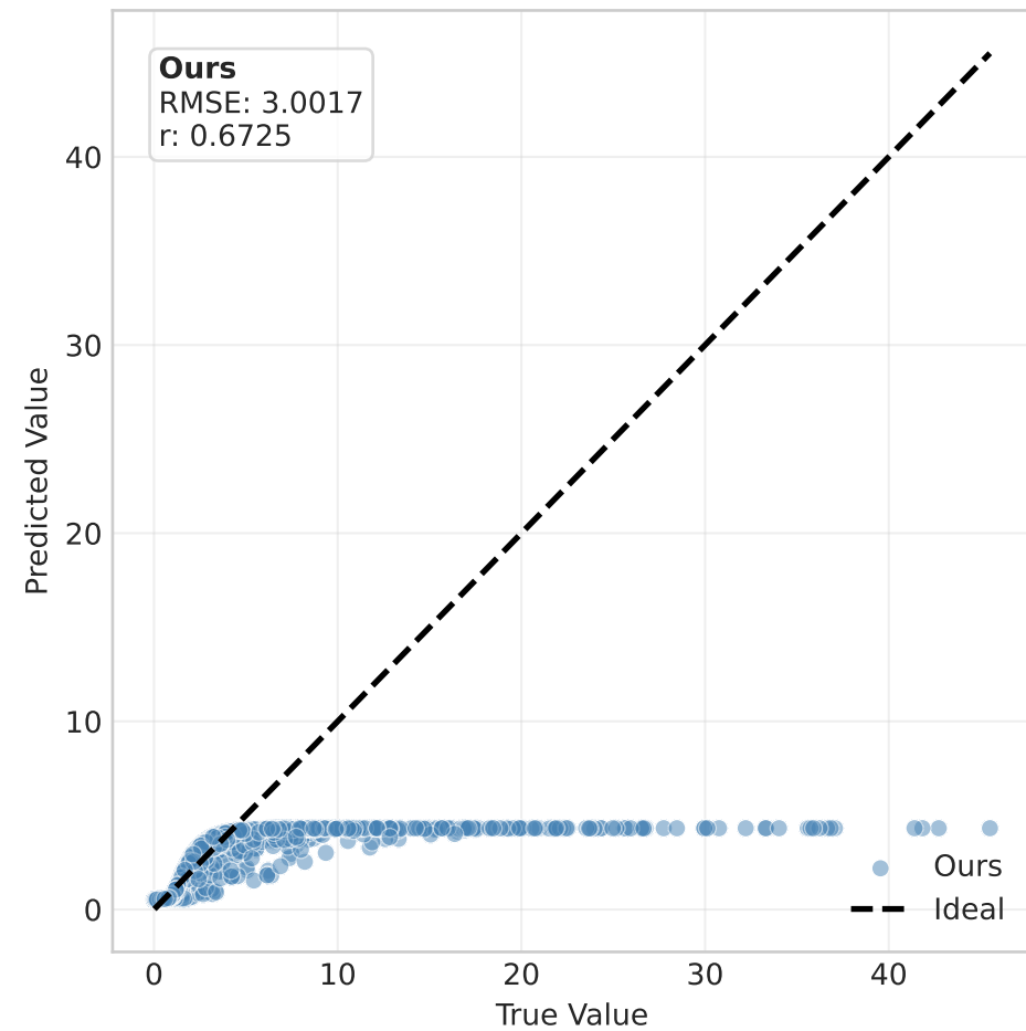
Basic Reproduction ( \mathcal{R}_0 )
