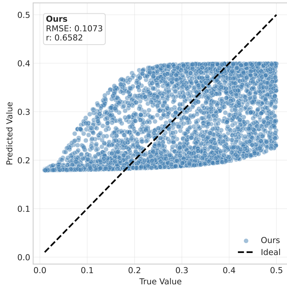
Infection Rate ( \beta )
