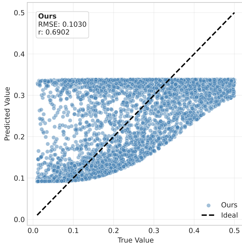
Recovery Rate ( \gamma )
