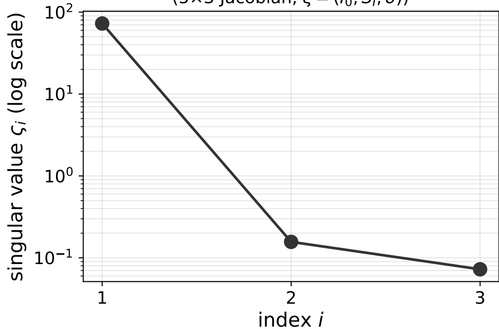
Restricted sampled-sensitivity spectrum ( 5 \times 3 Jacobian, \xi = (I_0, S_I, \sigma) )
