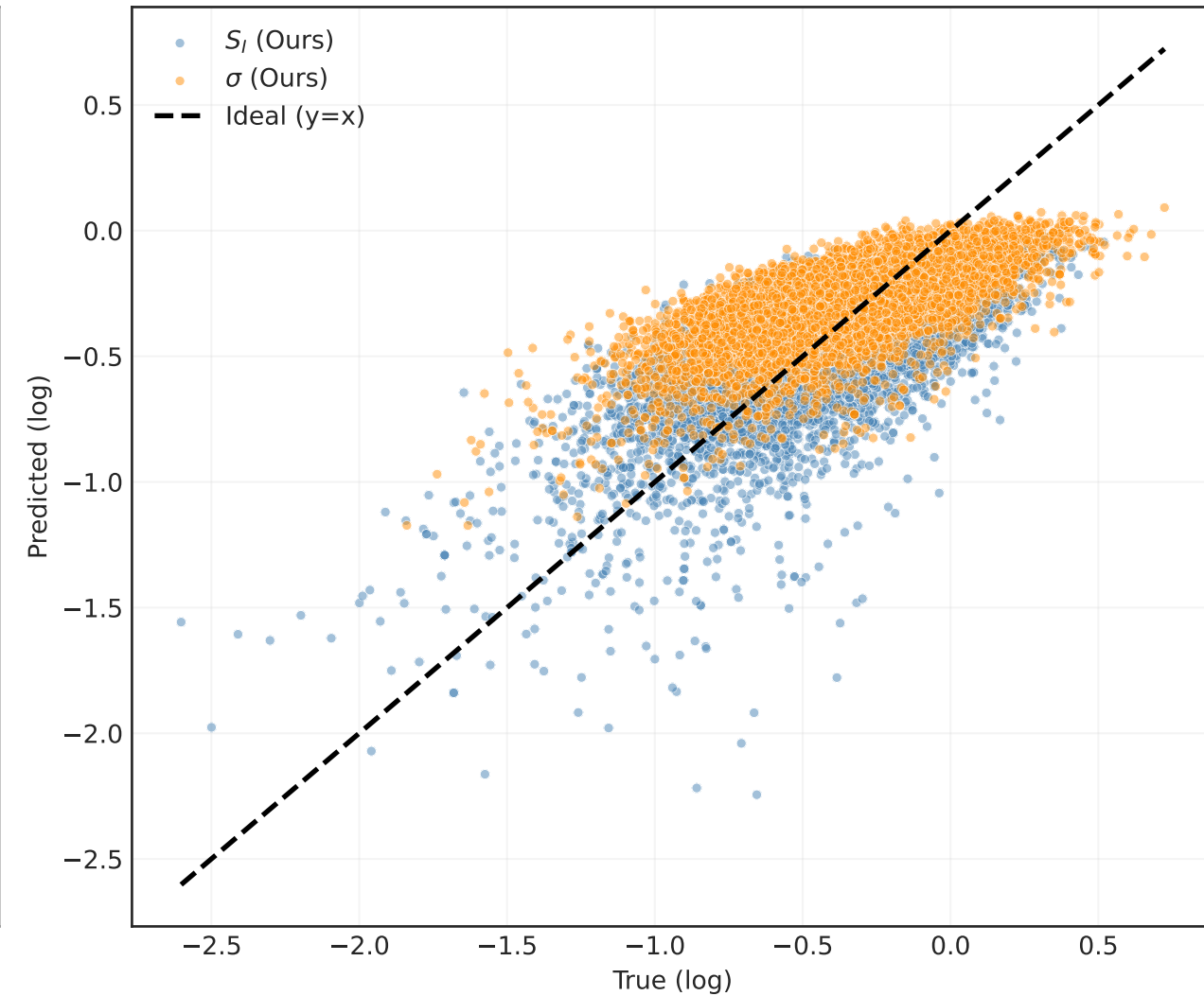
3. Individual coordinates S_l, \sigma (both weakly recovered)
