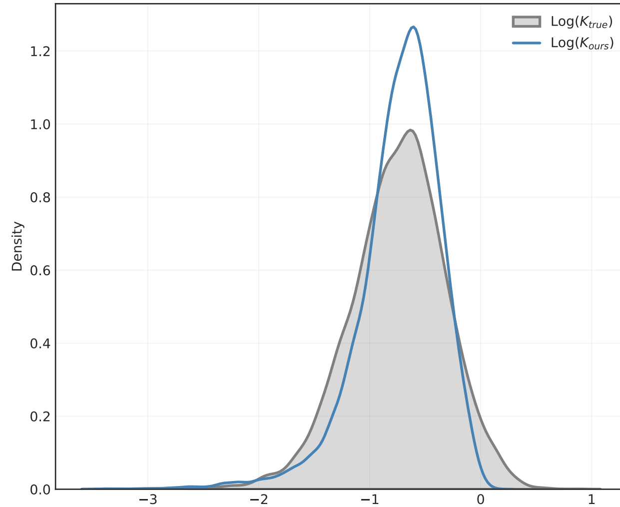
2. Product Consistency (Stiff Direction)
