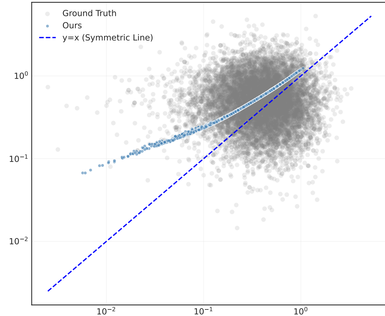
1. Log-Log Joint Distribution
