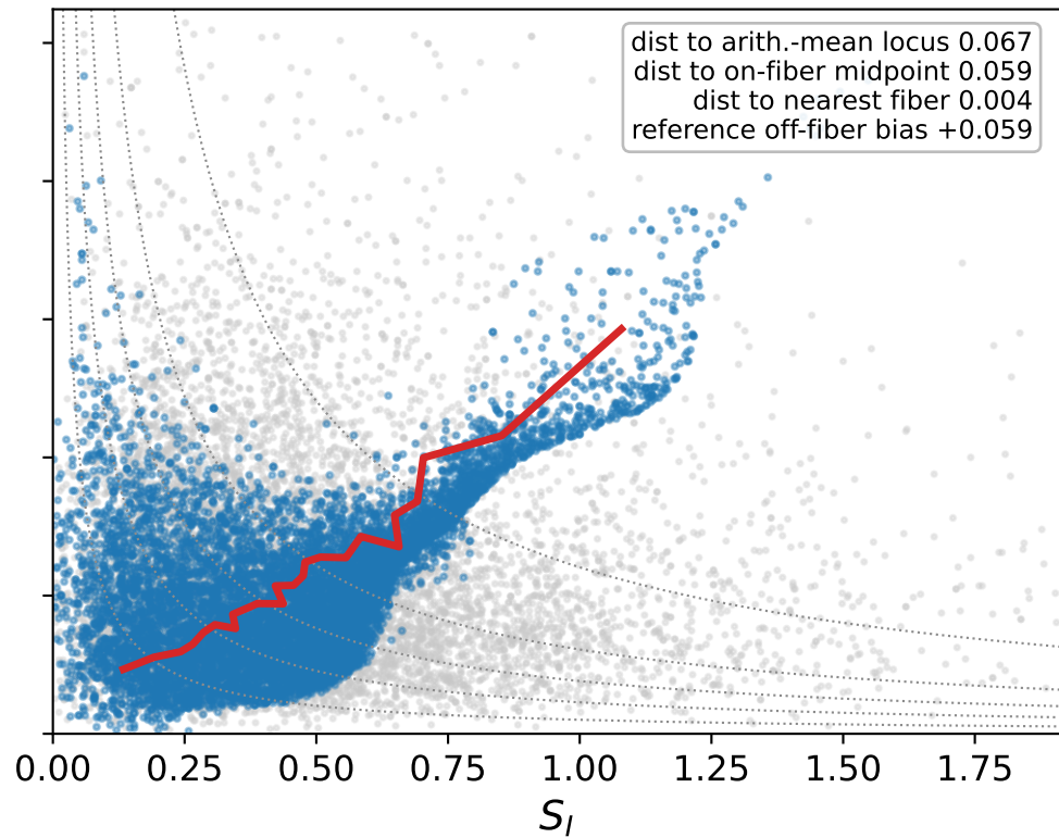
Direct estimator (matched)
