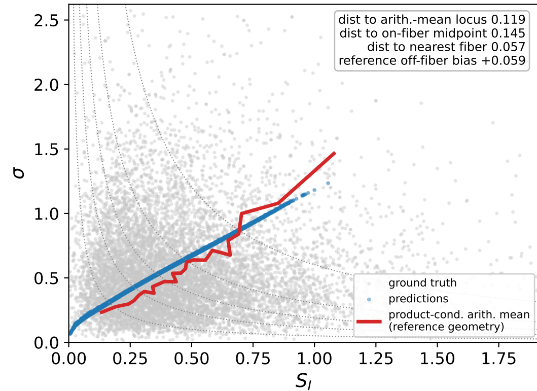
Iterative fixed point
