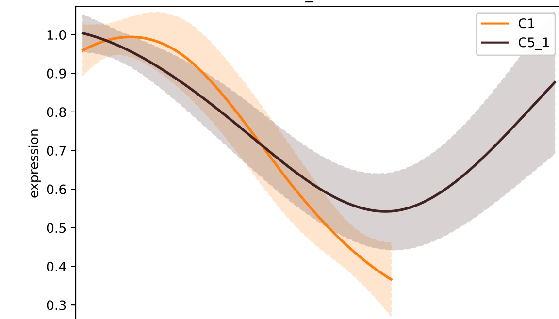
PF3D7_1239200
