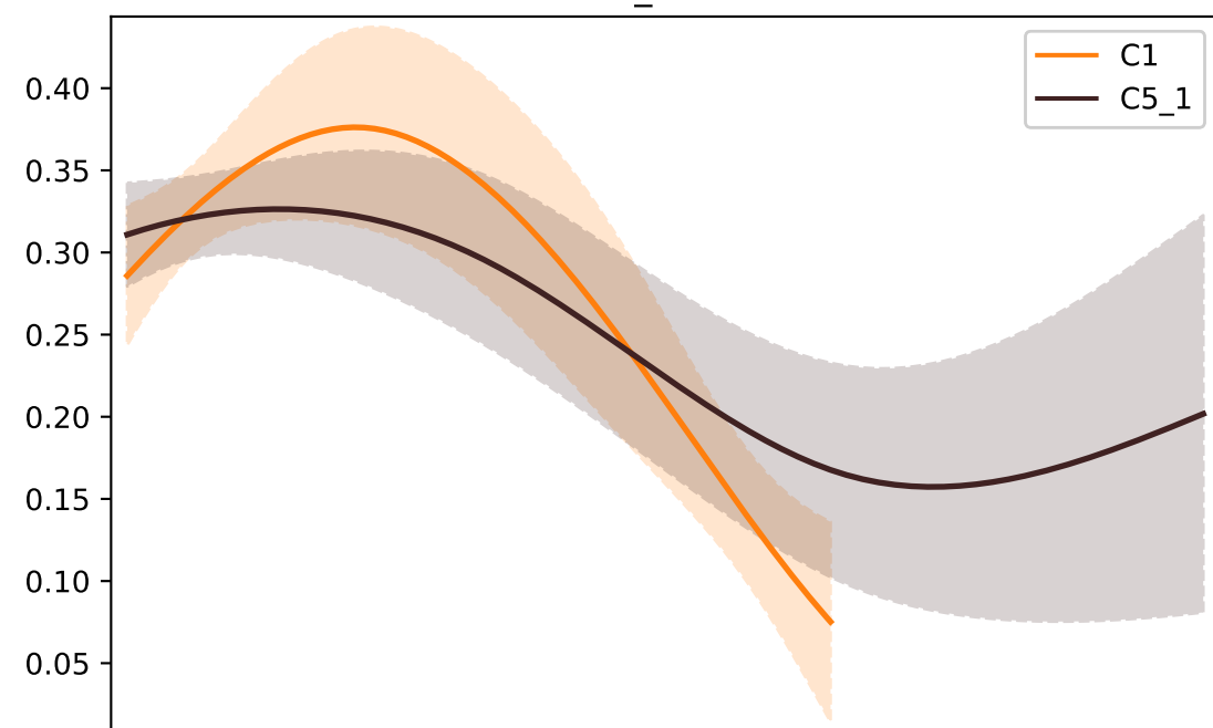
PF3D7_1350900
