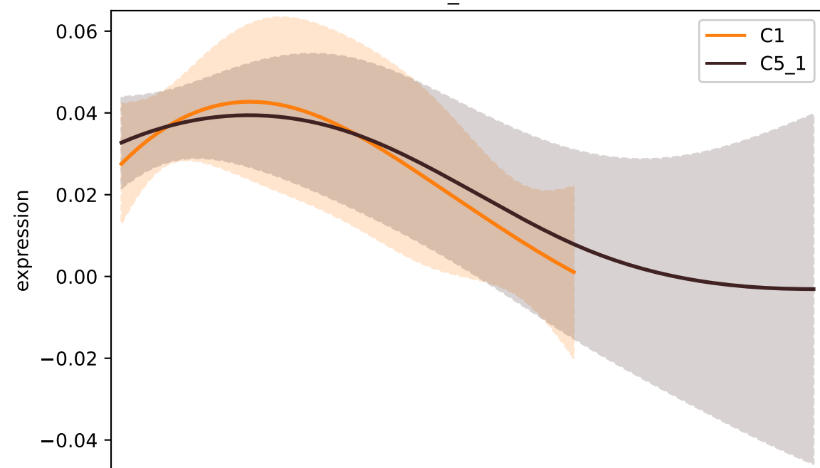
PF3D7_1408200
