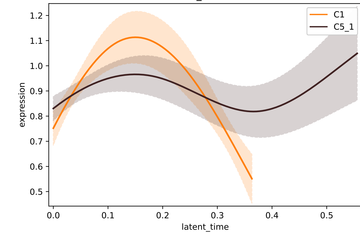
PF3D7_1239200
