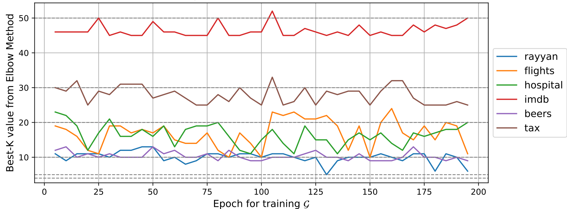
Epoch vs K Value Visualization
