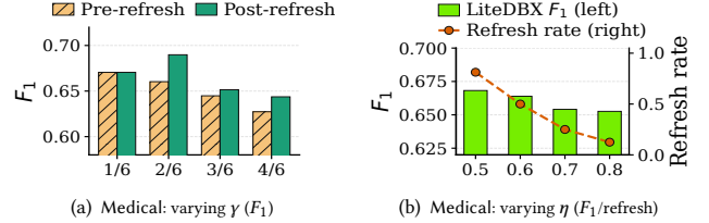
Figure 6: Varying update magnitude and tolerance.
