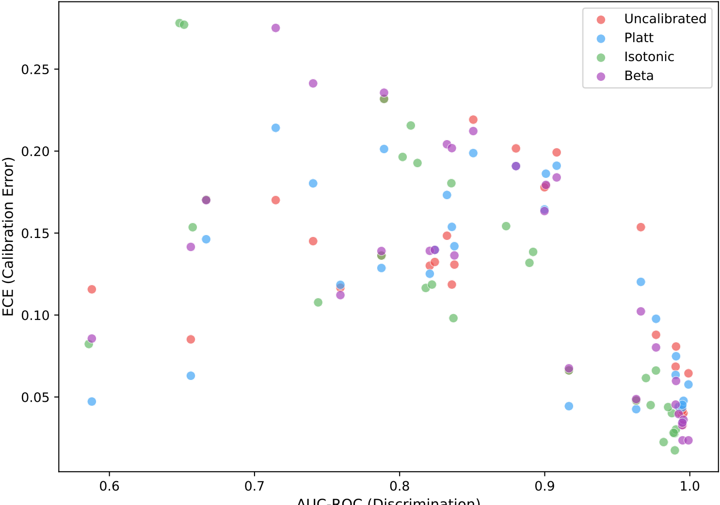
Figure 4: Discrimination vs. Calibration ( r=-0.573 , p=0.000 )
