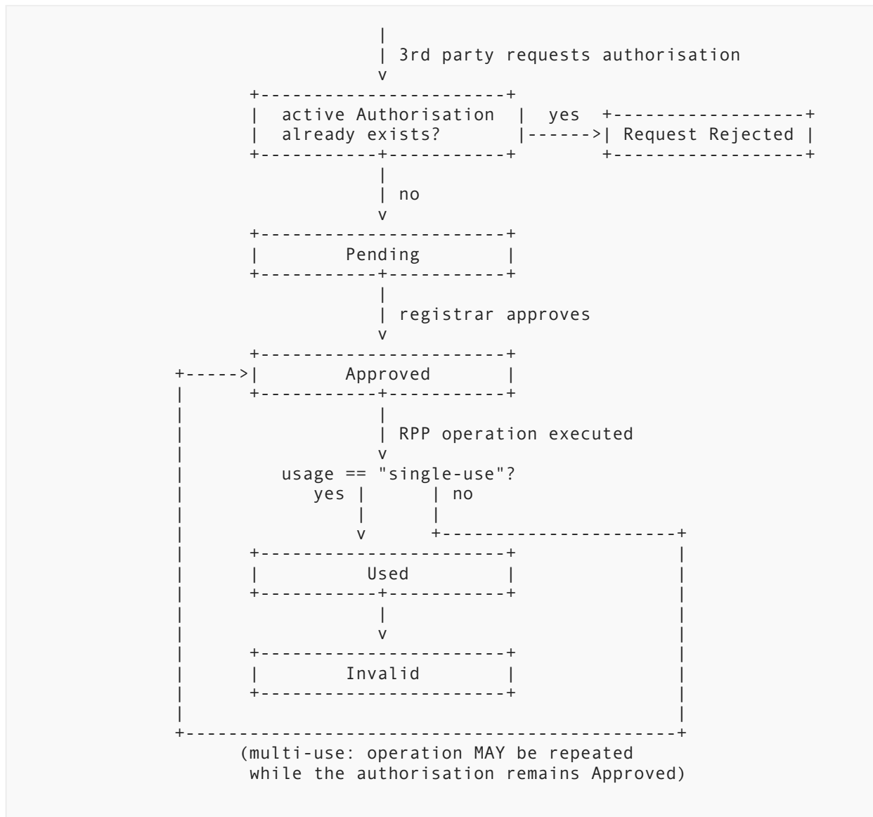
Figure 2: Authorisation Data Object lifecycle
