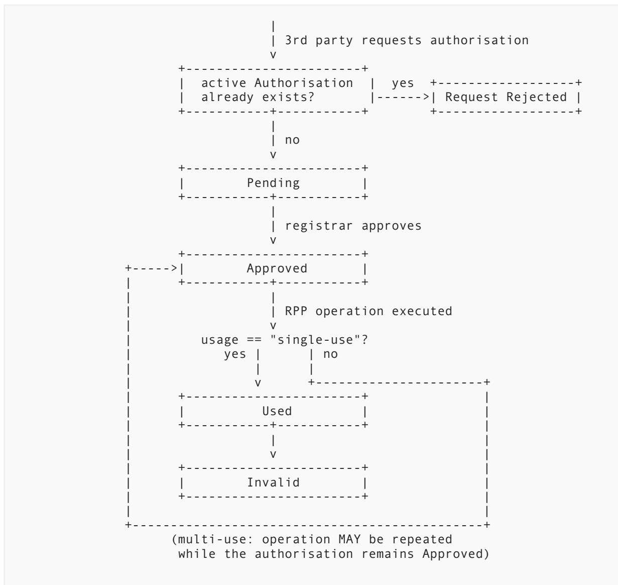
Figure 2: Authorisation Data Object lifecycle
