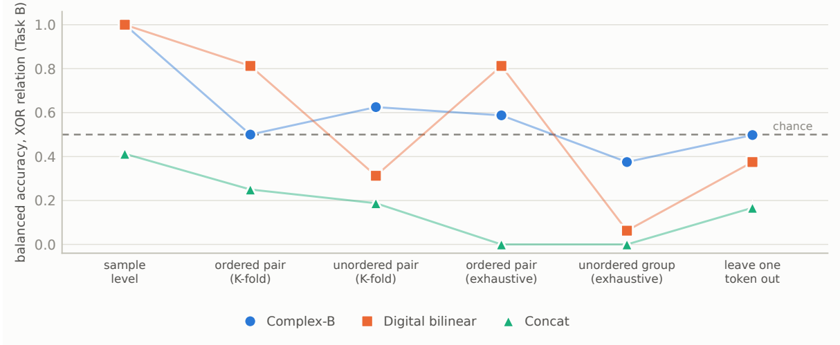
Figure 5: The XOR result depends on the unit of generalisation. Balanced accuracy on the parity relation under six splitting regimes, ordered from the released sample-level split (repeats of a pair split across folds) to leave-one-token-out. Shaded band marks \pm 0.06 around chance. The digital-bilinear peak at exhaustive ordered-pair grouping is a mirror-pair leakage artefact: z(x) \odot z(y) is symmetric, so the held-out pair’s mirror carries an identical feature vector. Lines join points of the same feature family and do not imply a continuum.
