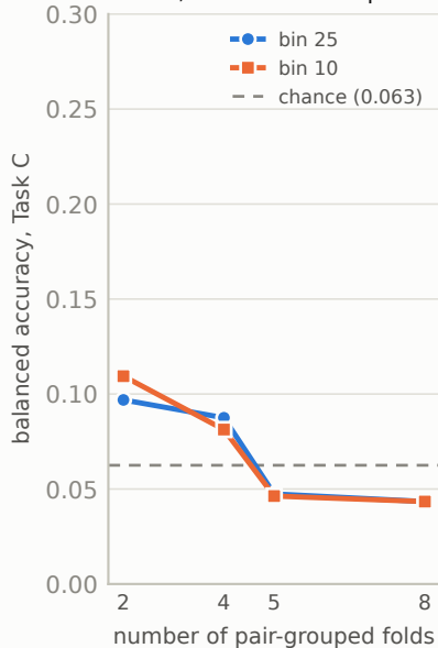
Task C, fold-count sweep
