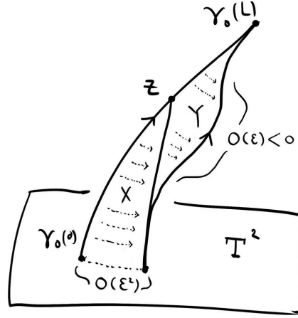
Figure 3: Intuitive idea of lemma 9
