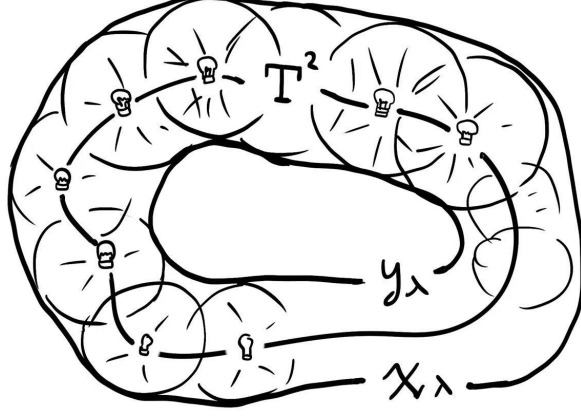
Figure 2: \mathcal{X}_\lambda, \mathcal{Y}_\lambda as wave fronts
