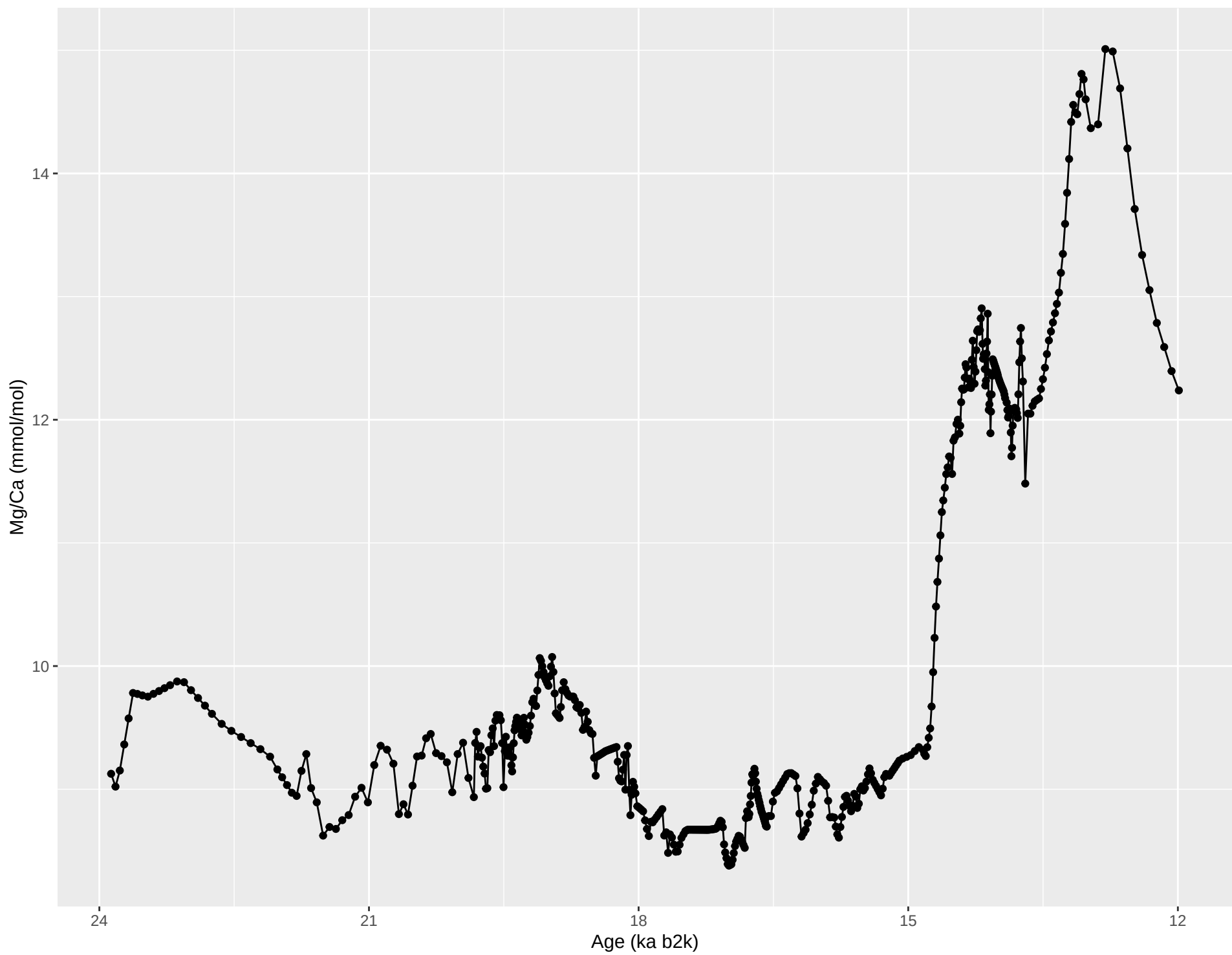
Mg/Ca vs age –Glas (Laura Endres)
