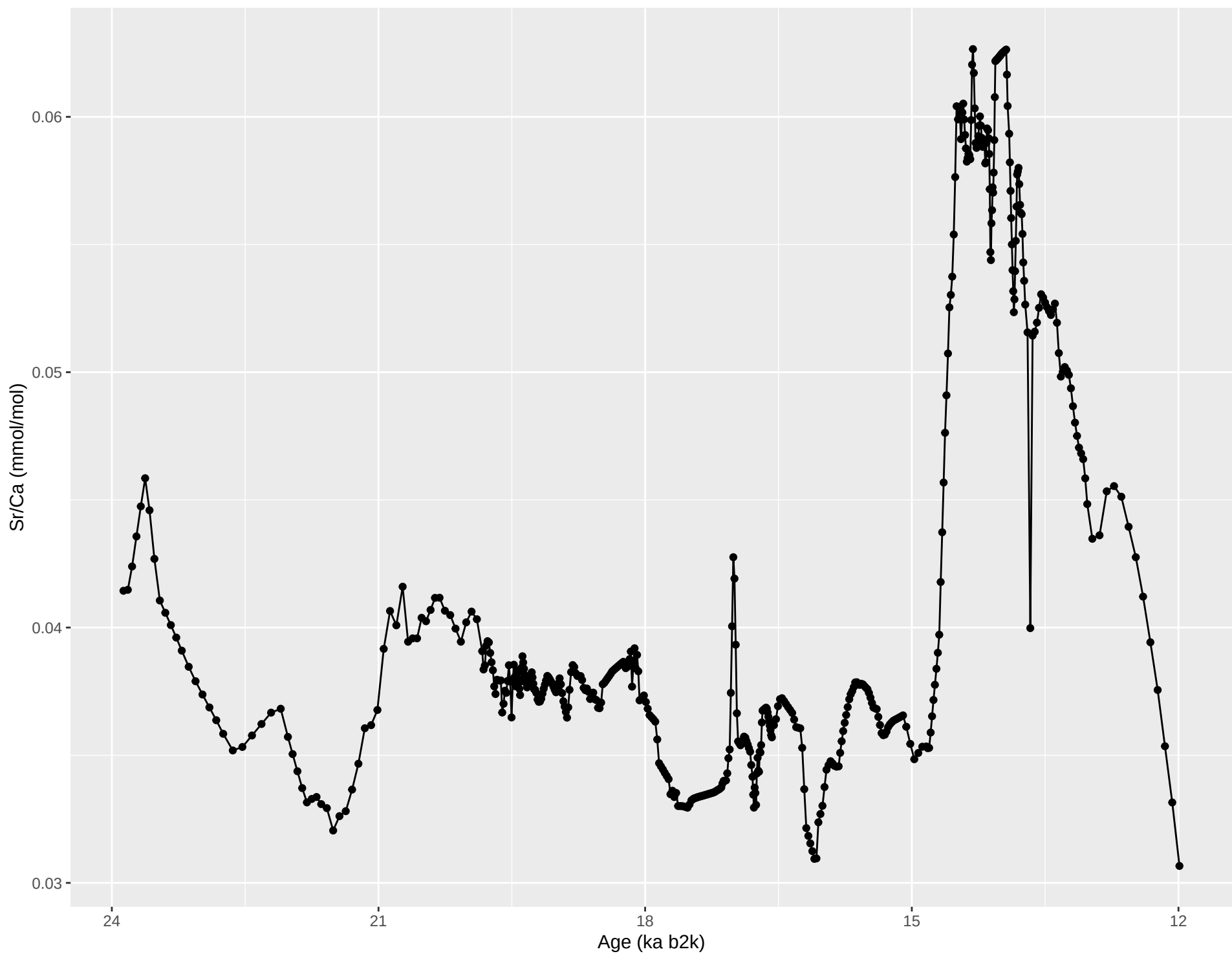
Sr/Ca vs age –Glas (Laura Endres)
