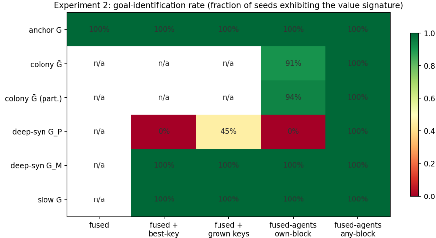
Figure 1: Experiment 2: fraction of seeds in which each planted goal exhibits the value signature, per convention (columns) and world (rows). ‘n/a’ marks recorded infeasibility (fused beyond \sim 10 variables; fused + best-key and fused + grown keys intake at colony scale). Any-block is the only column without a miss.
