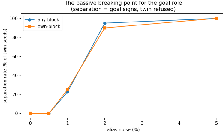
Figure 2: Experiment 3: separation rate (the goal exhibits the value signature, the twin does not) versus twin noise: the passive breaking point for the goal role lies between 1% and 2%.
