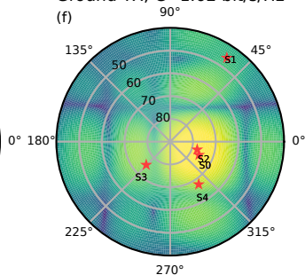
Ground TX, C=1.62 bit/s/Hz
