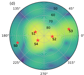
Ground TX Beampattern 5 Sats Capacity = 15.8 bit/s/Hz
