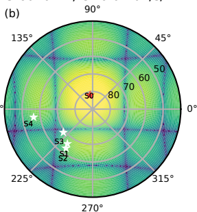
Ground TX, C=0.74 bit/s/Hz
