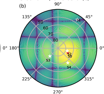
Ground TX, C=0.86 bit/s/Hz
