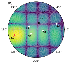
Ground TX Beampattern 5 Sats Capacity = 15.8 bit/s/Hz
