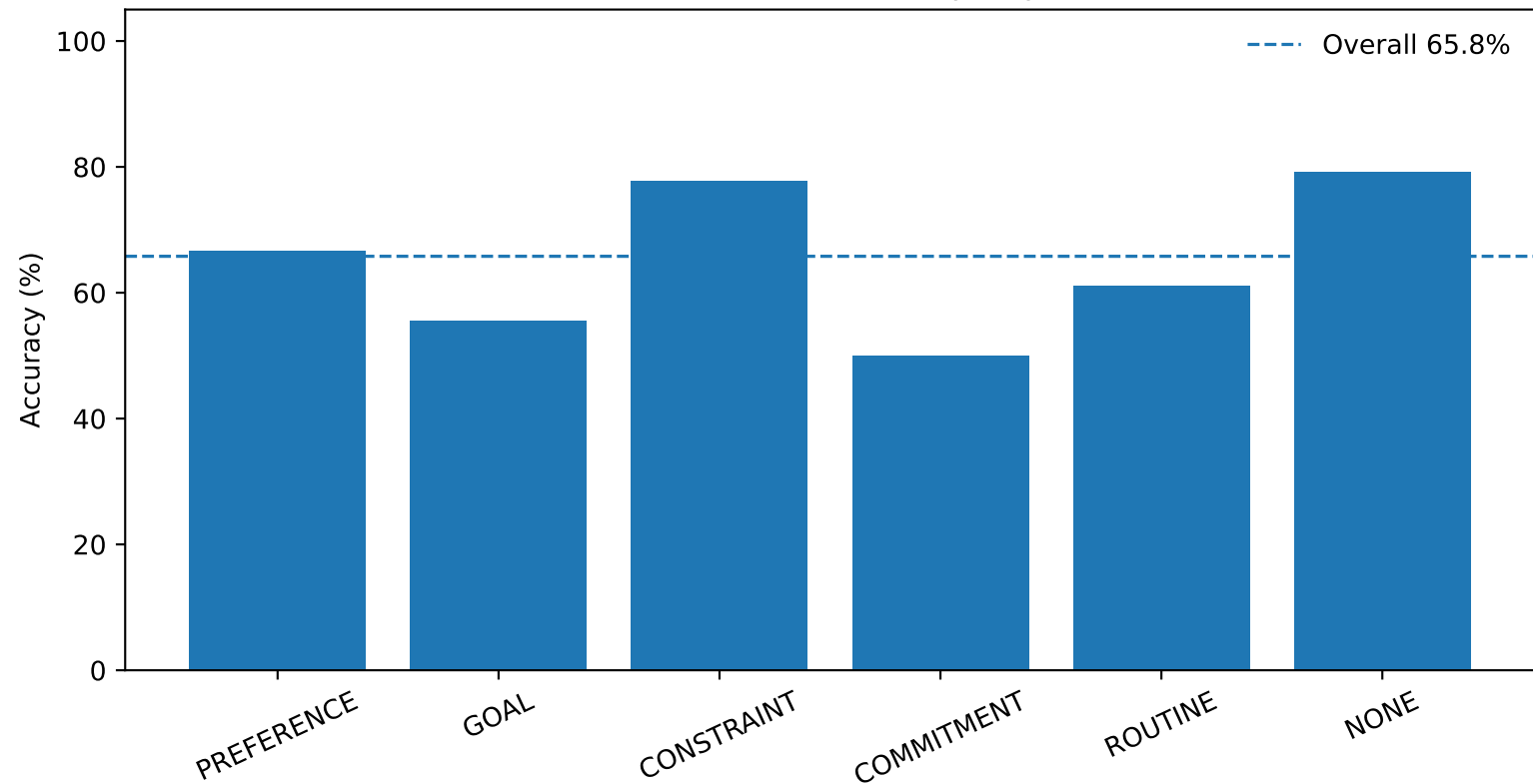
Observation router under held-out paraphrase families
