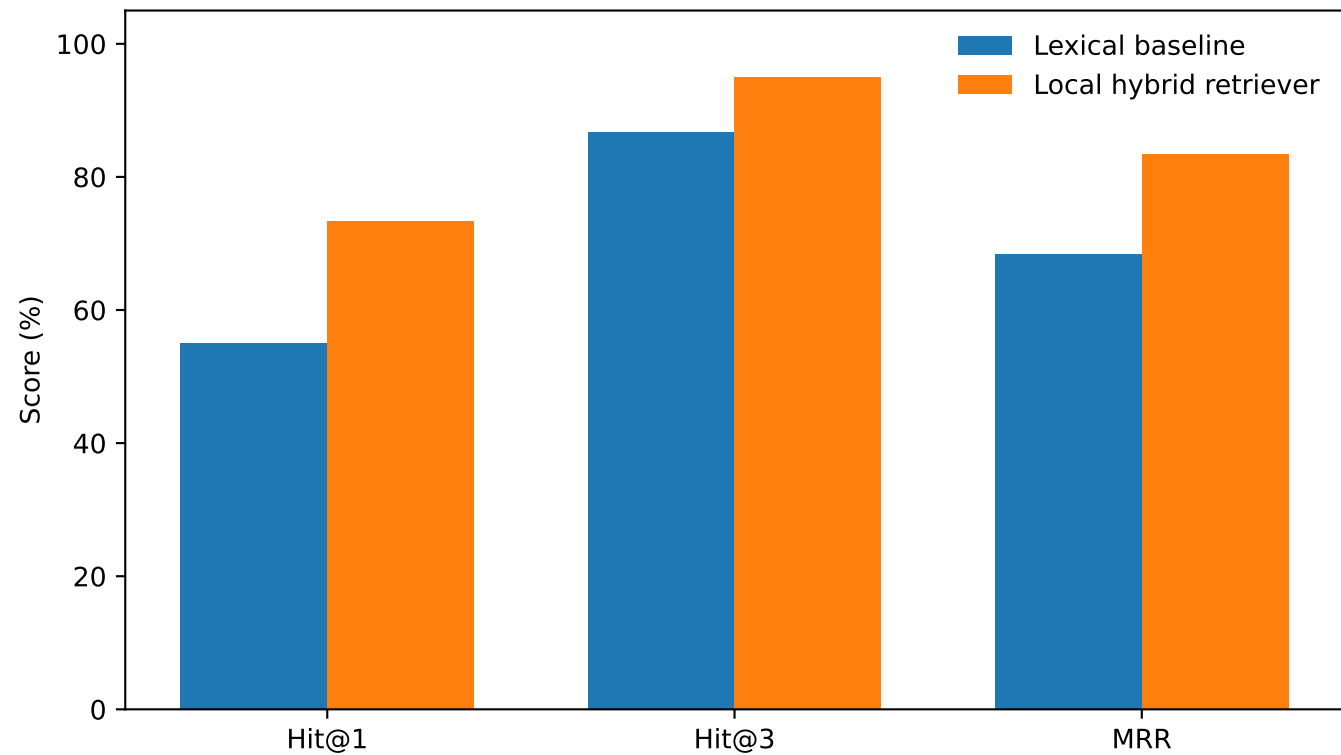
Retrieval benchmark (n=120)
