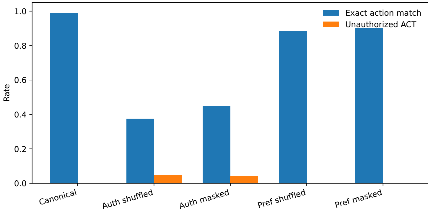
Negative controls isolate the role of authorization evidence
