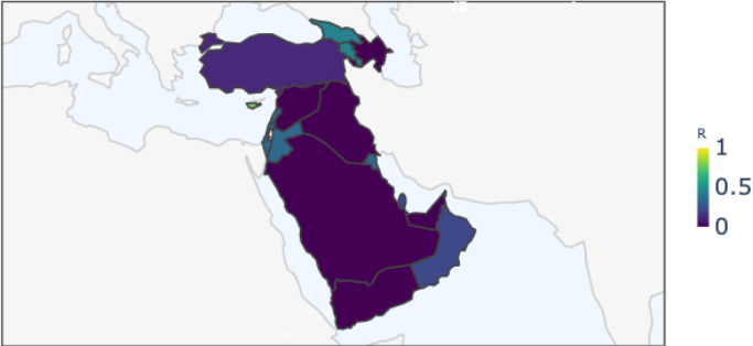
Western Asia Region — Enclosure Strength (R)
