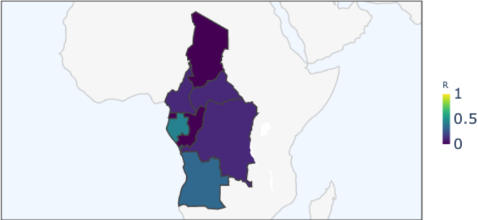
Middle Africa Region — Enclosure Strength (R)
