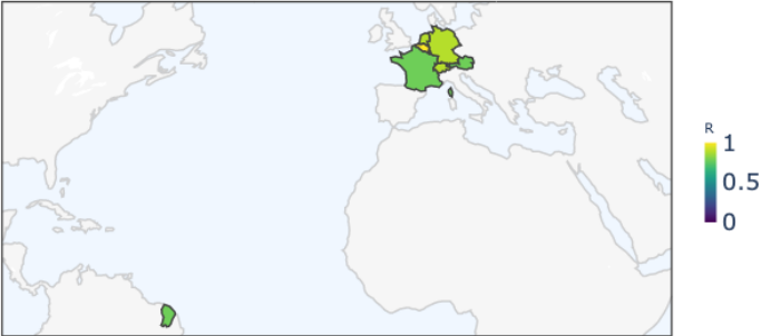
Western Europe Region — Enclosure Strength (R)
