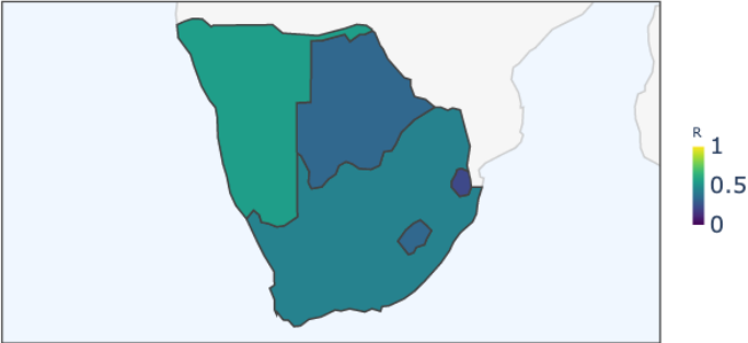
Southern Africa Region — Enclosure Strength (R)
