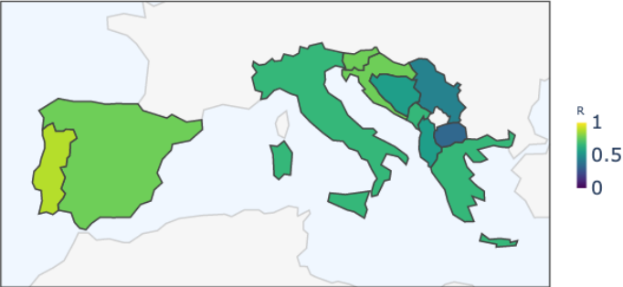
Southern Europe Region — Enclosure Strength (R)
