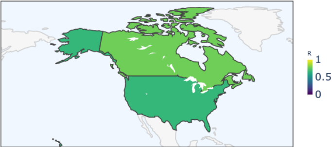
Northern America Region — Enclosure Strength (R)
