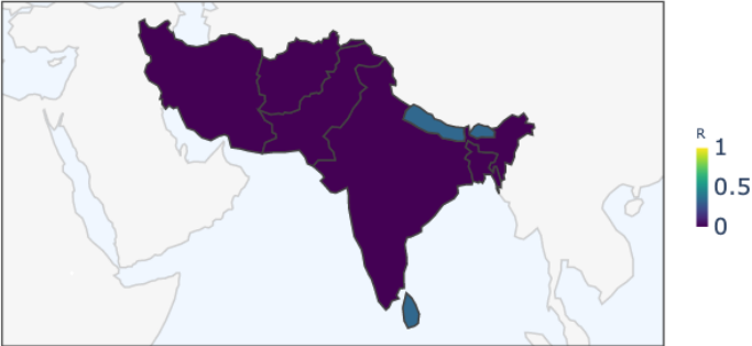
Southern Asia Region — Enclosure Strength (R)
