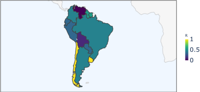
South America Region — Enclosure Strength (R)
