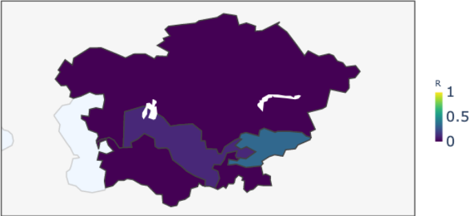
Central Asia Region — Enclosure Strength (R)
