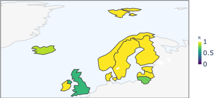
Northern Europe Region — Enclosure Strength (R)
