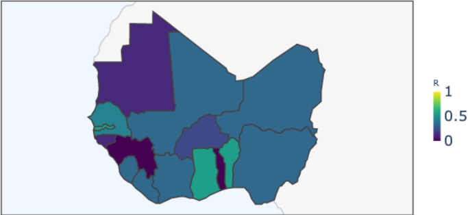
Western Africa Region — Enclosure Strength (R)
