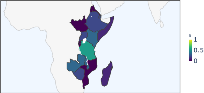
Eastern Africa Region — Enclosure Strength (R)
