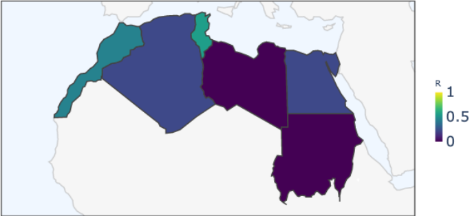
Northern Africa Region — Enclosure Strength (R)
