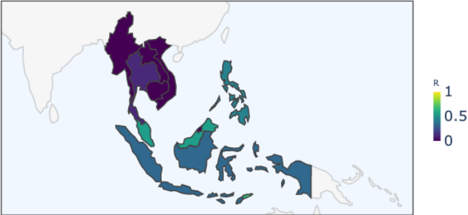
South-eastern Asia Region — Enclosure Strength (R)
