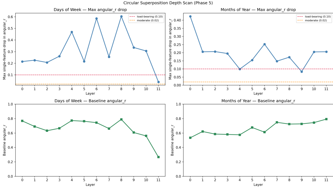
Figure 10: Layer-wise circular superposition scan for days of the week (left) and months of the year (right). Top row: maximum single-feature ablation drop in r_{\text{angular}} per layer. Bottom row: baseline r_{\text{angular}} per layer.
