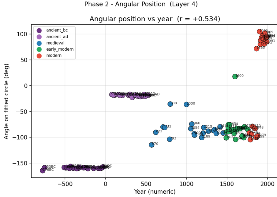
Figure 3: Angular position on fitted circle vs numeric year at layer 4 ( r = +0.534 ). Points coloured by epoch category.
