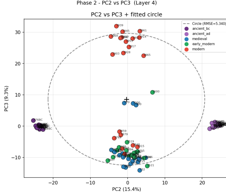
Figure 2: PC2 vs PC3 at layer 4 with algebraic circle fit (RMSE = 5.340).
