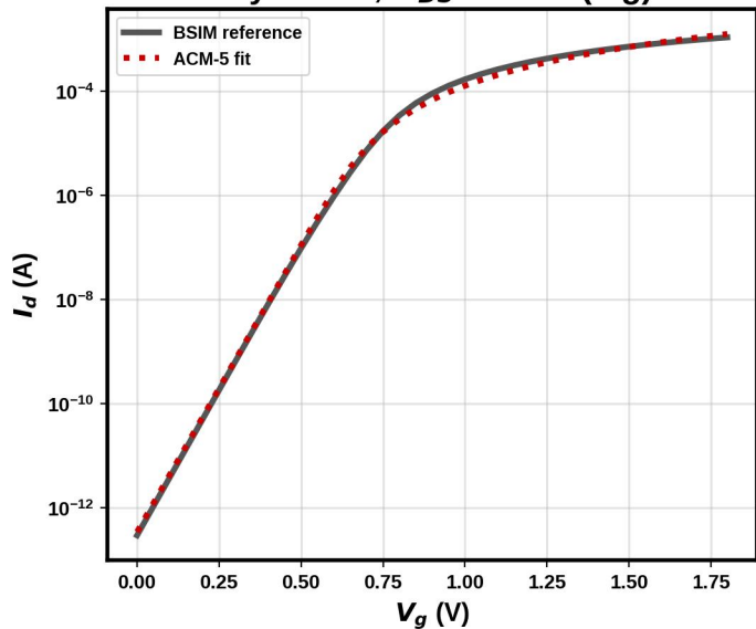
sky130 TT, V_{DS} = 1.8 V (log)
