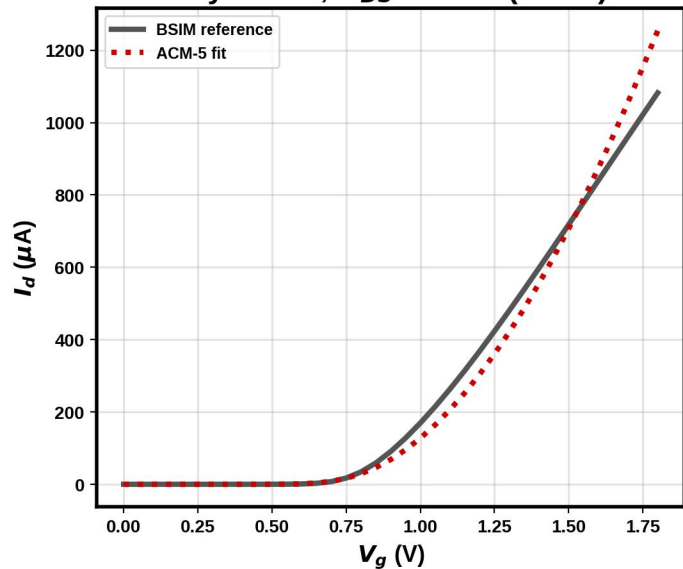
sky130 TT, V_{DS} = 1.8 V (linear)
