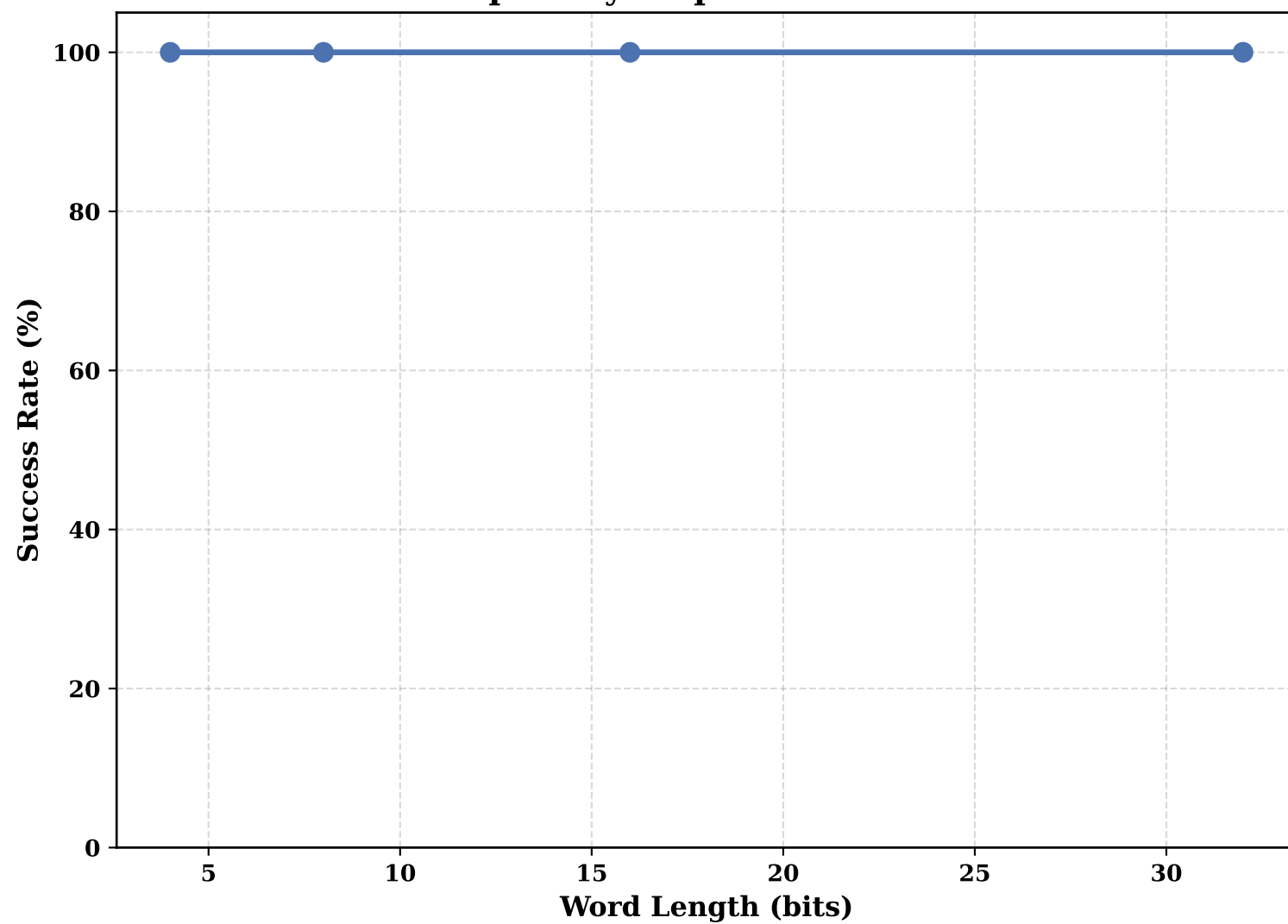
HammingSECDDECC
