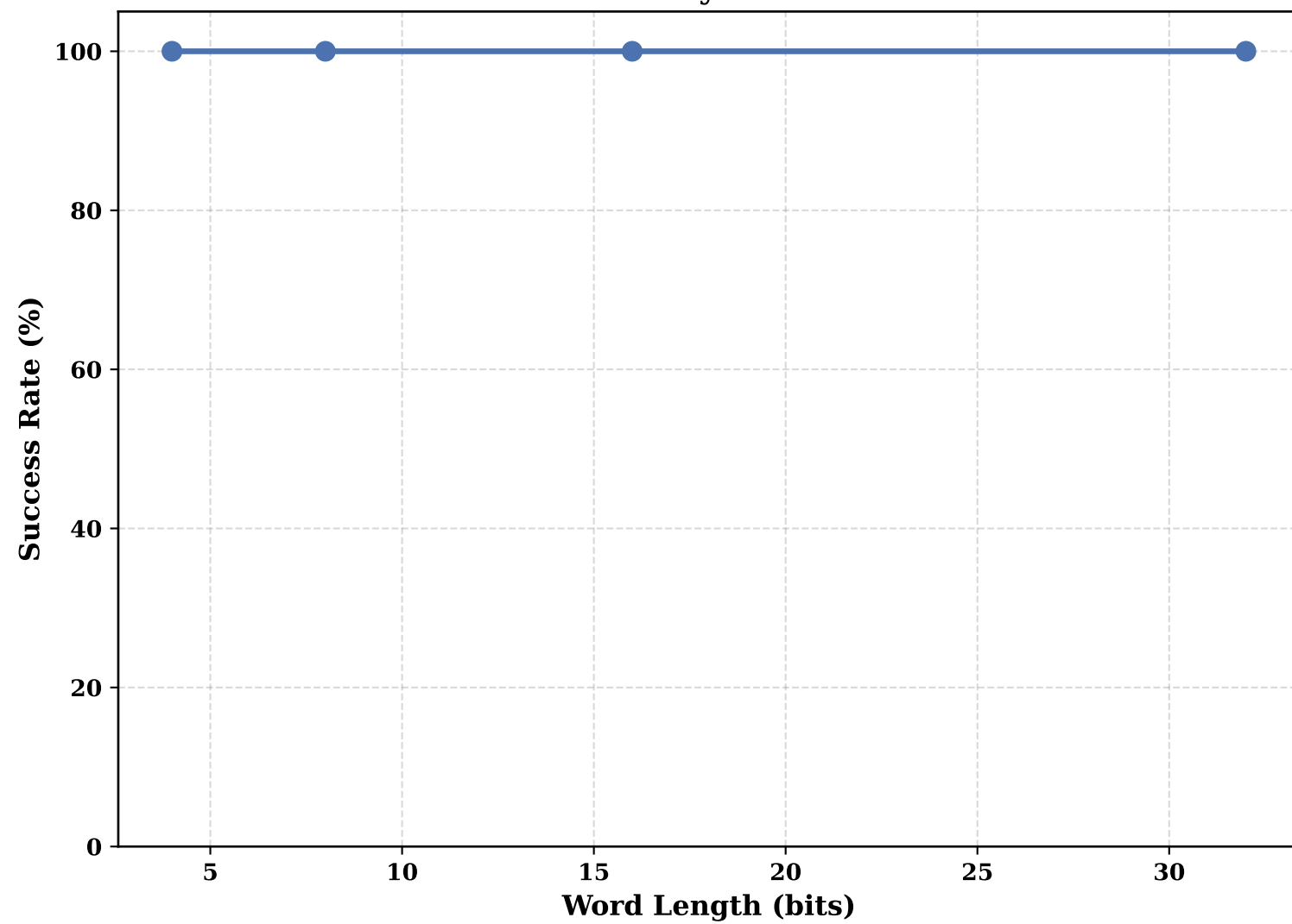
NonBinaryLDPCCECC
