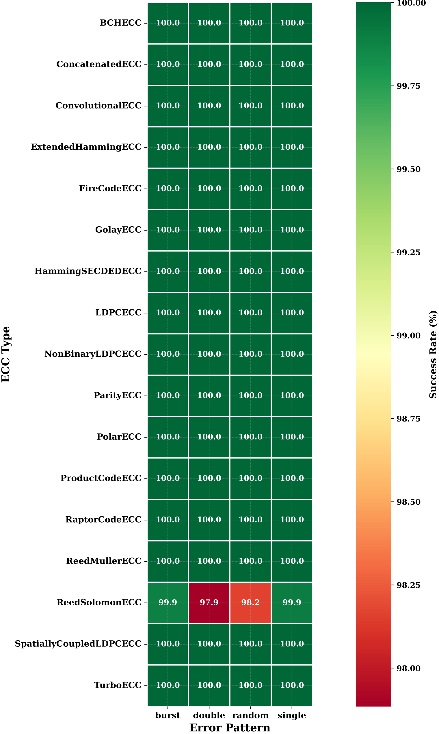
ECC Performance Heatmap by Error Pattern
