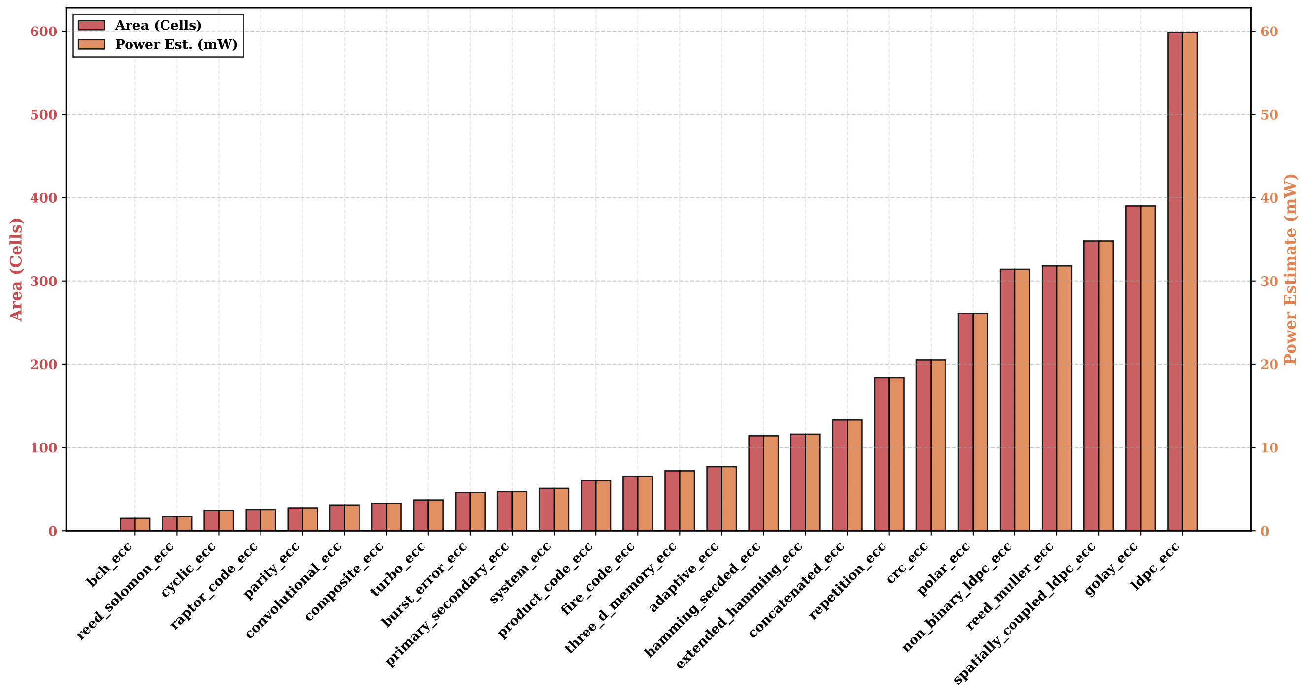
Hardware Cost Comparison: Area and Power
