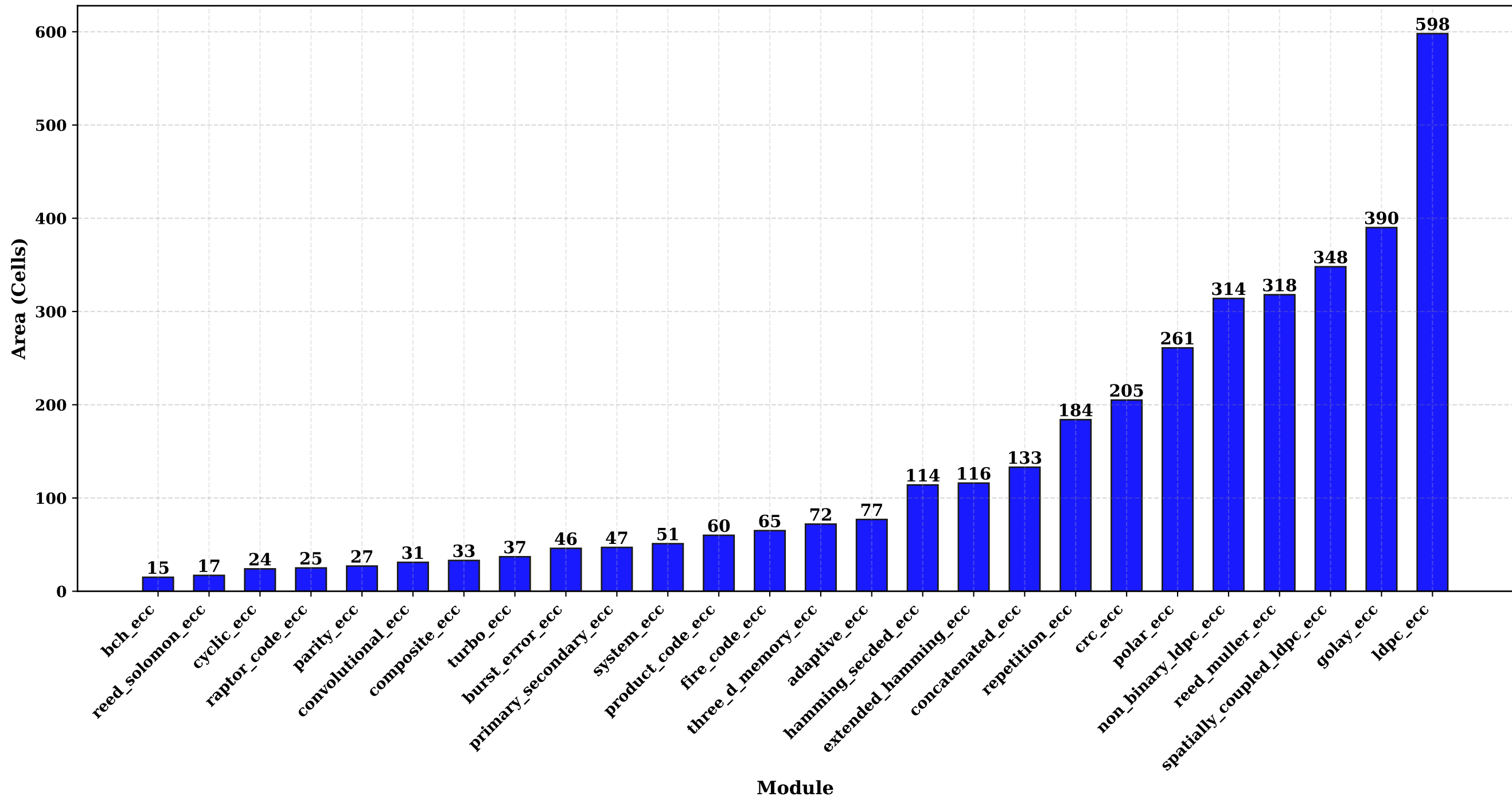
Hardware Cost Comparison: Area (Cells)
