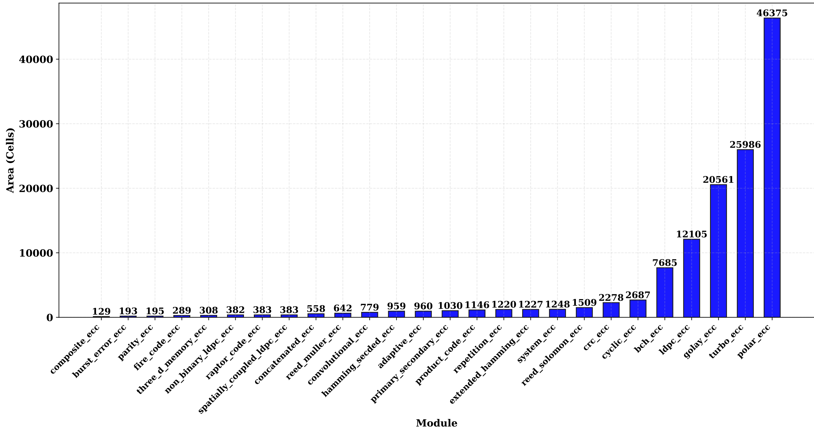
Hardware Cost Comparison: Area (Cells) - 64-bit Data Width
