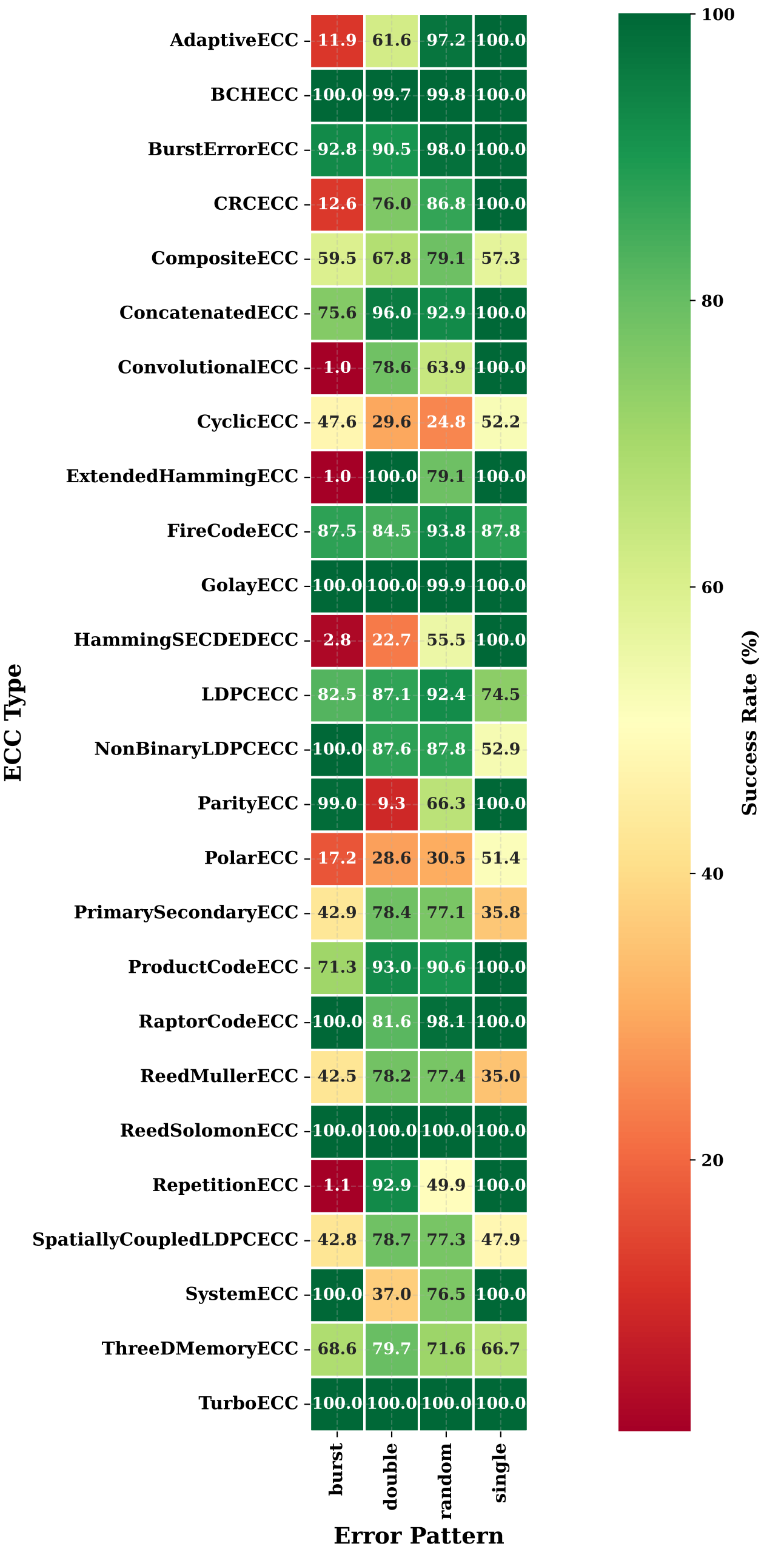
ECC Performance Heatmap by Error Pattern
