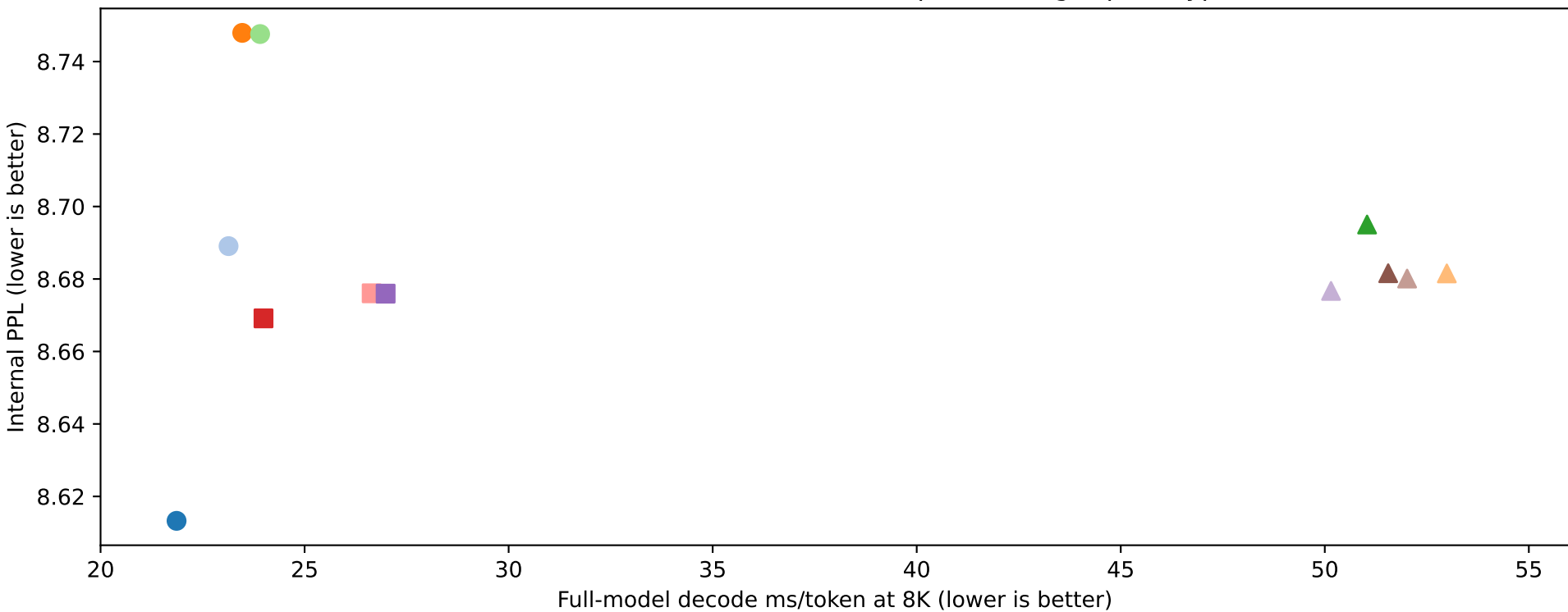
Frozen Qwen2.5-1.5B, 4/336 heads replaced; eager prototypes
