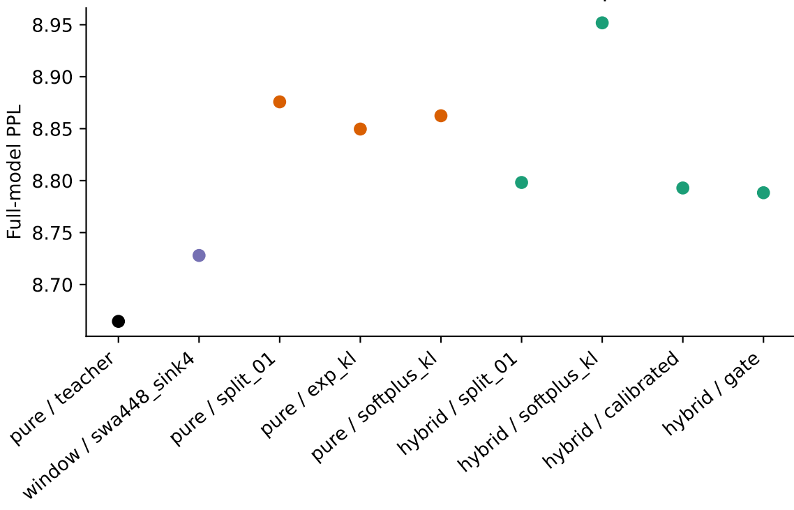
Wiki, 1024 tokens; 24/336 heads replaced
