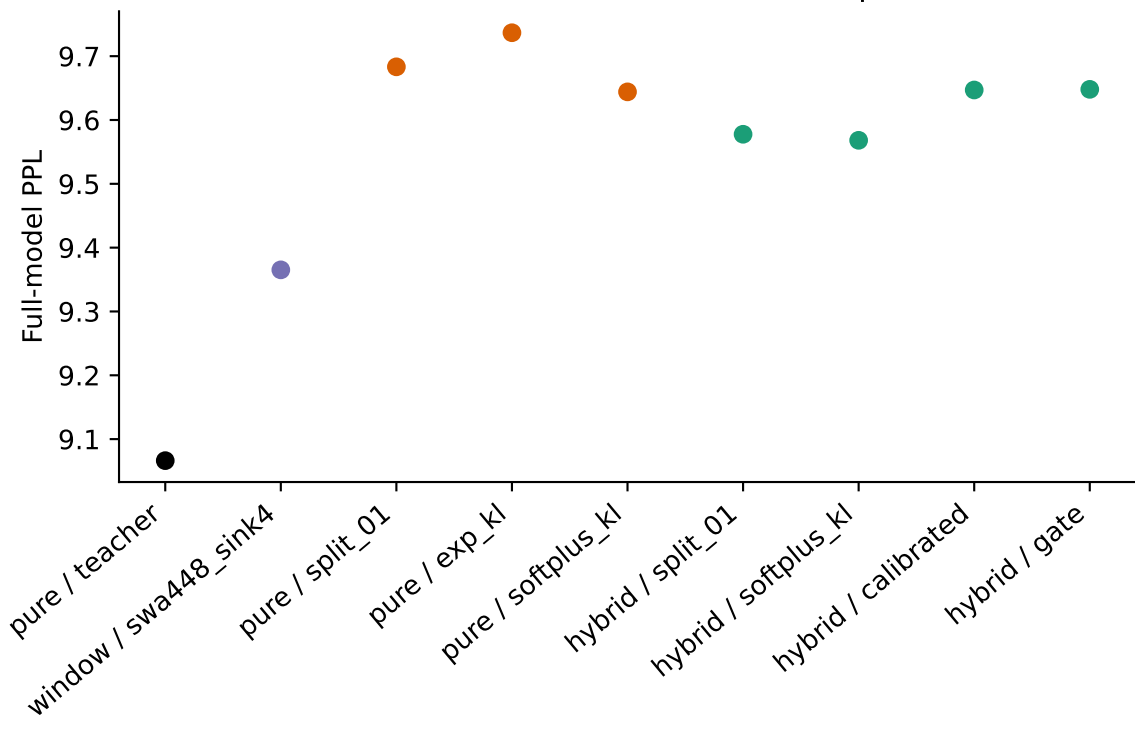
Wiki, 8192 tokens; 24/336 heads replaced
