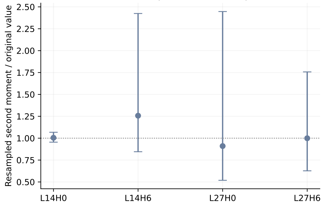
Document bootstrap: 2.5 / 50 / 97.5 percentiles
