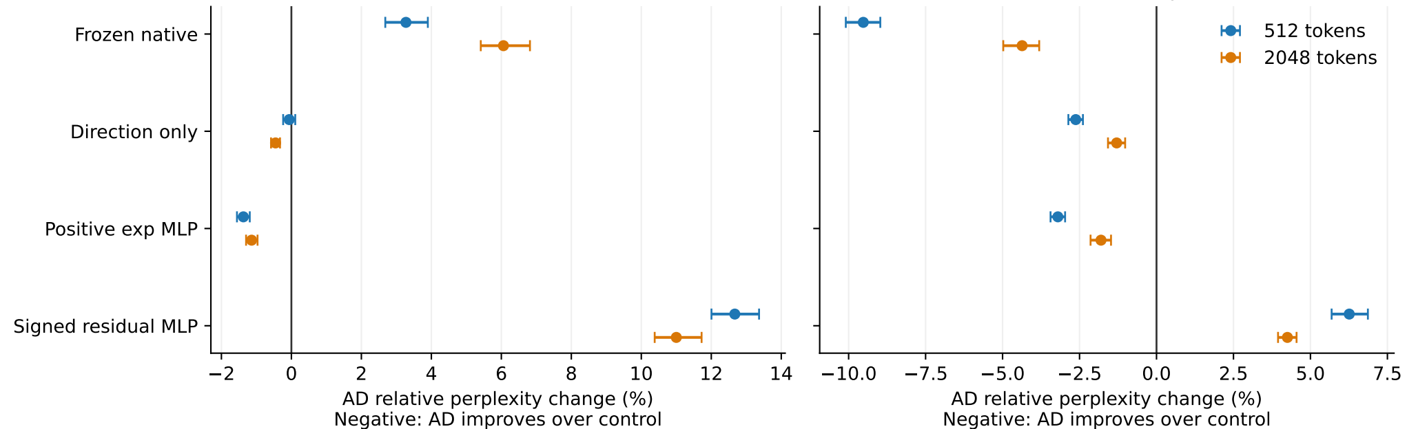
GDN: AD write amplitude
