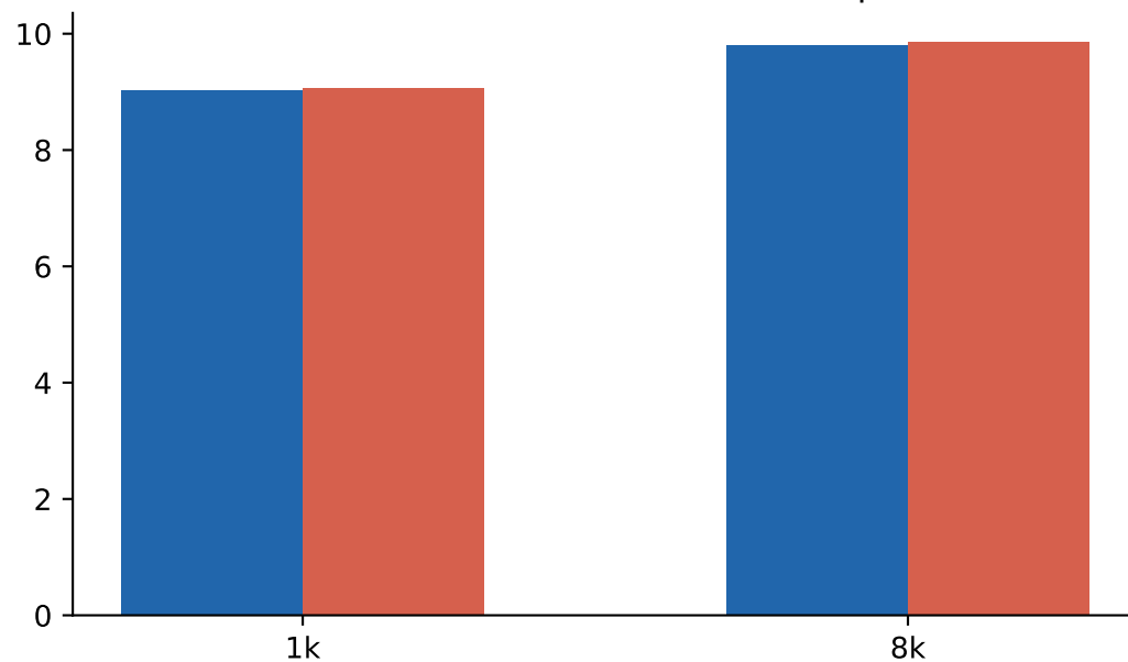
Frozen model PPL: 24/336 heads replaced
