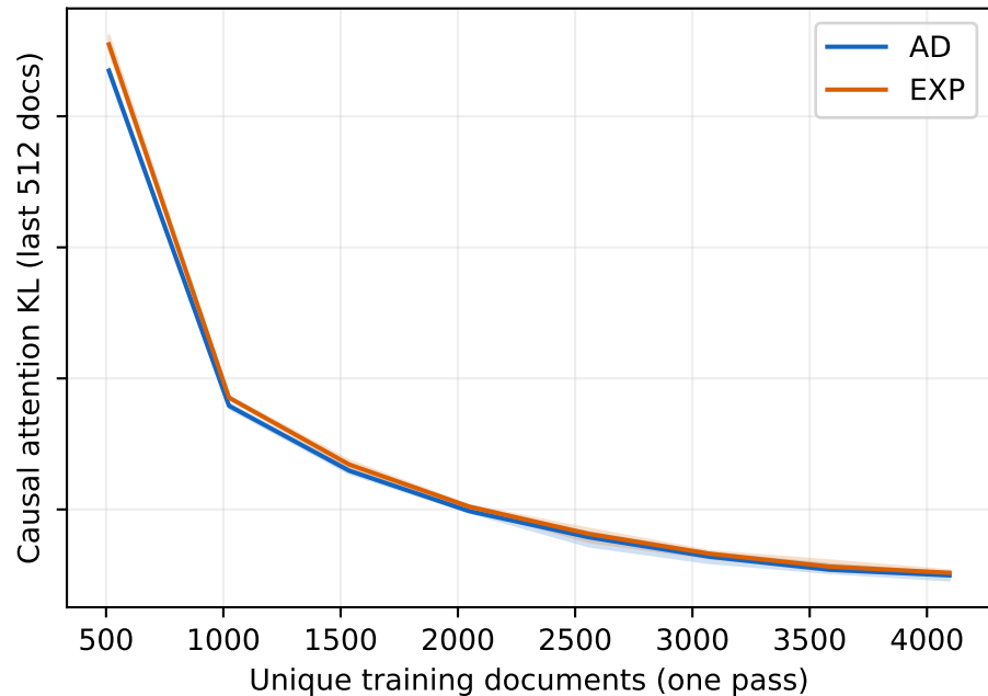
Same initial normalized attention
