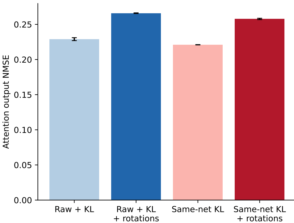
Fresh Wiki 1024 tokens
